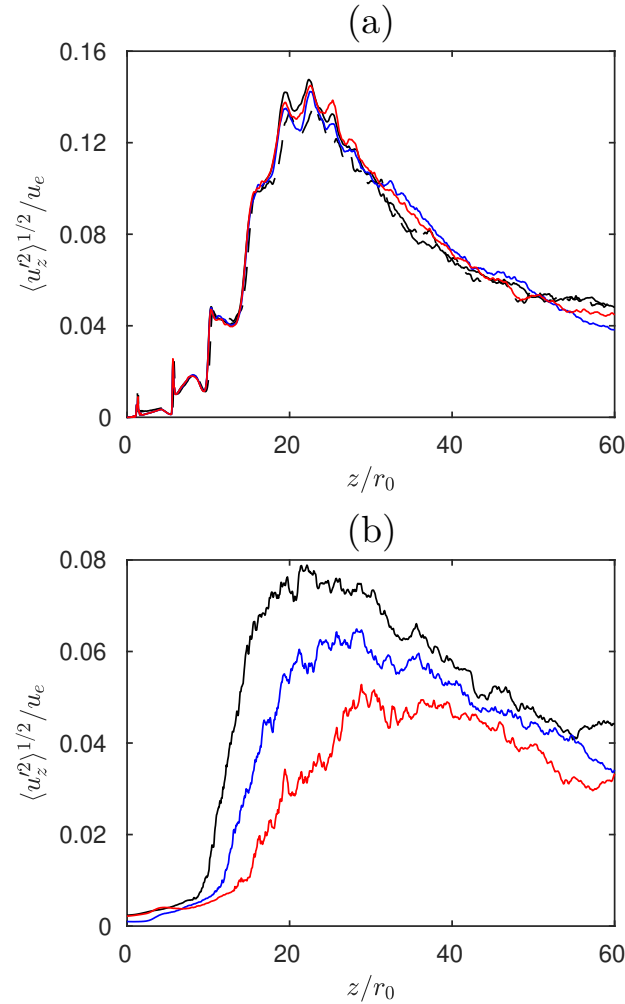
FIG. 6. RMS value of velocity fluctuations on (a) the jet axis and (b) in the center of the jet midplane for — Twinh2D, — Twinh2.4D, — Twinh2.8D and - - - SingleJet.
