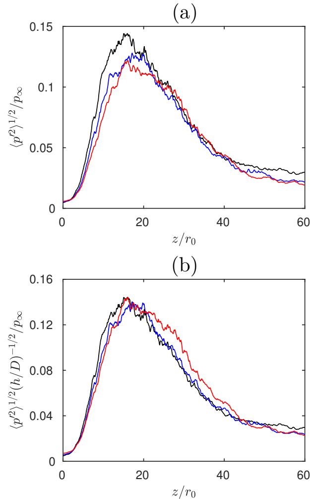
FIG. 12. RMS values of the pressure fluctuations in the jet midplane normalized by (a) p_\infty and (b) (h/D)^{1/2} p_\infty for — Twinh2D, — Twinh2.4D and — Twinh2.8D.
