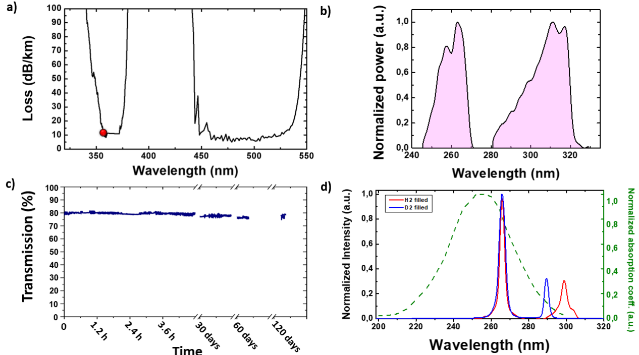
Fig. 1: (a) Cutback measurement results. The red spot represents the result from a cut back made with a 355 nm laser. (b) Normalized transmissions in the UV measured with a plasma lamp. (c) Fiber lifetime measurement under UV radiation over 120 days. (d) Raman generation plots in a 25 cm D 2 -filled fiber (blue curve) and in a 7 cm H 2 -filled fiber (red curve). The green curve represents the normalized absorption coefficient of the ozone in the Hartley band.
