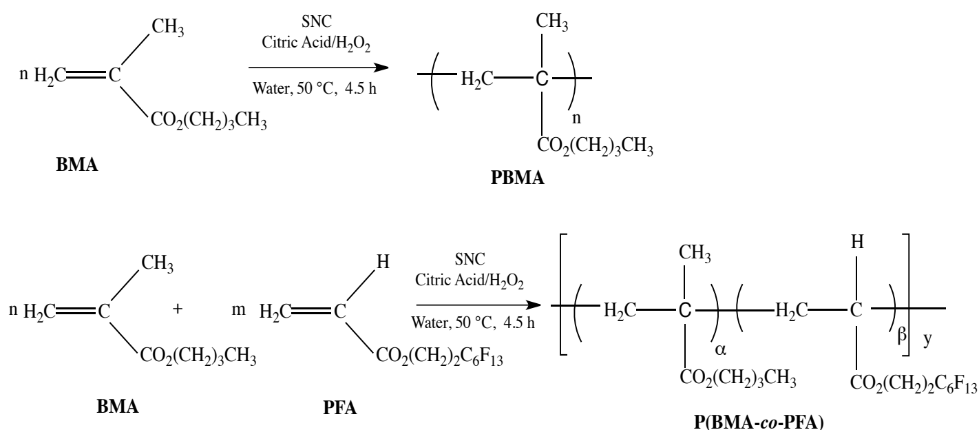
Scheme 1: Radical emulsion homopolymerization of BMA, and copolymerisation of BMA with PFA initiated by H 2 O 2 /Citric acid in deionized water ([BMA] 0 / [PFA] 0 = 90/10 in the feed) (SNC stands for starch nanocrystal as pickering stabilizer emulsion).
