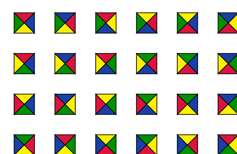
Fig. 1 - Tileset \mathcal{T} of 24 tiles.
