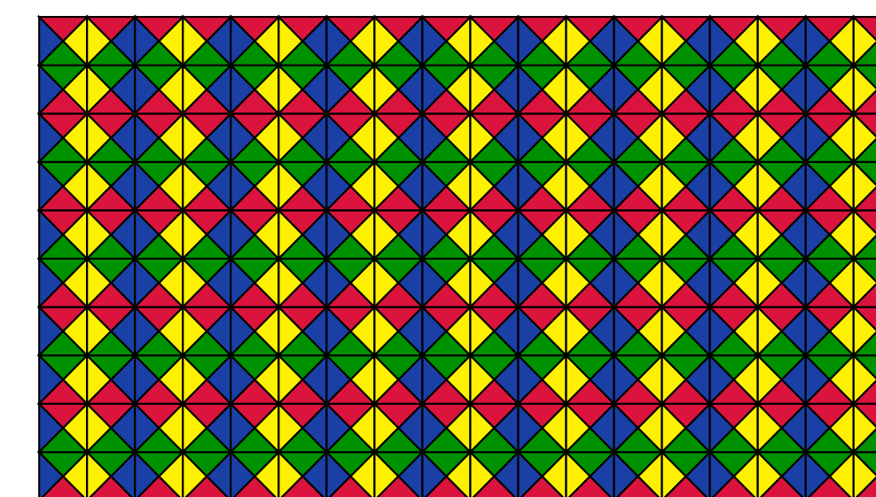
Fig. 2 - Example of a valid tiling with some tiles of \mathcal{T}
