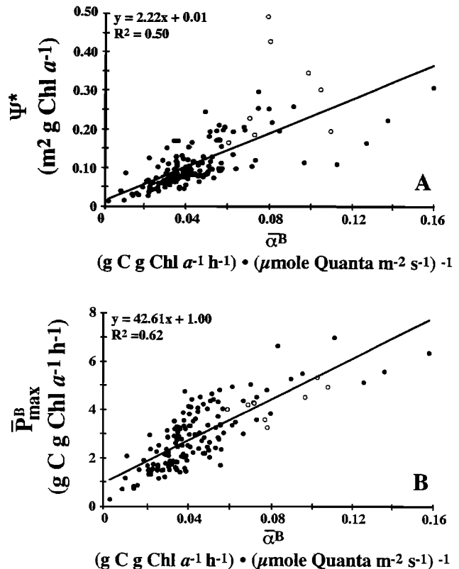
Figure 14. \Psi^* and photophysiological parameters at Palmer stations B and E, Antarctica: (a) Relationship between \alpha^B and \Psi^* . (b) relationship between \alpha^B and \bar{P}_{max}^B . Open circles indicate ice-covered waters; solid circles indicate ice-free waters.
