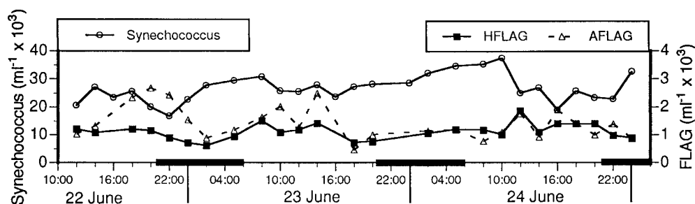
Fig. 1. Temporal changes in concentrations of HFLAG, AFLAG, and Synechococcus in the Bay of Villefranche. Dark bars denote nighttime hours.
