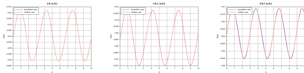
FIGURE 19. Simulations for l = 0 , l = 0.2 and l = 0.5 - shifted and non-shifted Hamiltonian integrator - h = 0.1
