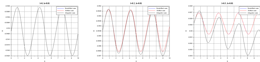
FIGURE 21. Simulations for l = 0 , l = 0.2 and l = 0.5 -comparison of the value of the first integral for the shifted , non-shifted Hamiltonian and Challamel's integrator - h = 0.01
