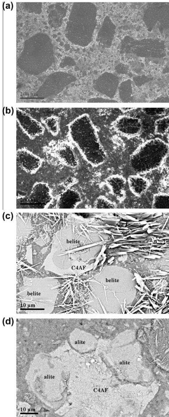
Fig. 6. Micrographs of UHPC4 and UHPC5 samples. (a and b) Secondary electron images: homogeneous versus heterogeneous crushed quartz repartition. In UHPC5, crushed quartz is preferentially fixed to the sand. (c and d) Back-scattered electron images: residual clinker. Belite is very visible in UHPC4 and difficult to find in UHPC5.
