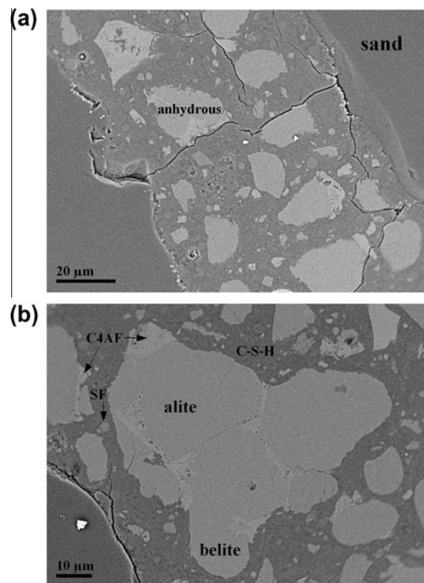
Fig. 3. Back-scattered electron images of UHPC1 sample (polished sections): (a) sand and paste with many anhydrous clinker grains. (b) Polymineralic grain of clinker containing alite, belite and C 4 AF (light grey), silica fume noted SF (middle grey), and C-S-H (dark grey).
