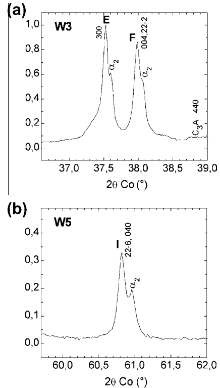
Fig. 5. Powder X-ray diffraction of the cement investigated in this study. The angular windows (a) W3 and (b) W5, as defined by Courtial et al. [30], exhibit the characteristic lines (E, F and I) of the M1 polymorph of alite. The hkl indexes are related to the \langle M \rangle Pc unit cell as described by de Noirfontaine et al. [29].
