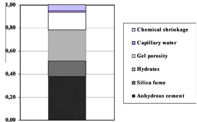
Fig. 2. Volumetric phases distribution of a UHPC according to the Powers-Jensen model.
