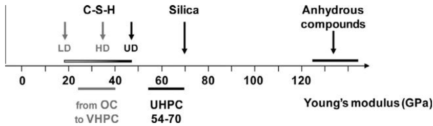
Fig. 7. Variation range of the Young's modulus. Under the axis: our samples (black) compared to the other types of non UHPC concretes (grey). Above the axis: the Young modulus of the various components of a concrete. The values are the values given by Velez et al. [33], Sorelli et al. [25] and Vandamme et al. [34].
