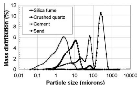
Fig. 1. Particle size distribution of the UHPC components, measured by laser granulometry.
