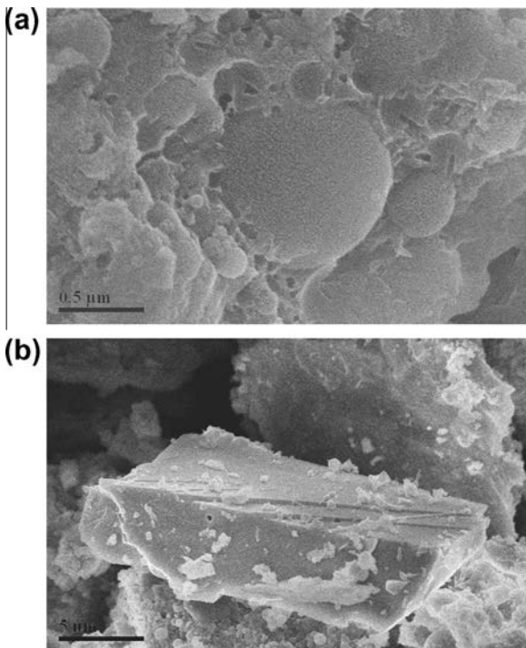
Fig. 4. Secondary electron images in the UHPC3 paste (fractures): (a) silica fume and C-S-H hydrates and (b) crystal of alite, silica fume and hydrates.
