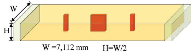
Fig. 11. Rectangular waveguide bandpass filter with vias.
