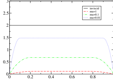
Figure 1: Viscous solution u_\mu(x) given by (1.26), (1.27) for L = 1 , \alpha = 1 , f = 4 , and different values of the viscosity \mu . The black line is the inviscid solution.
