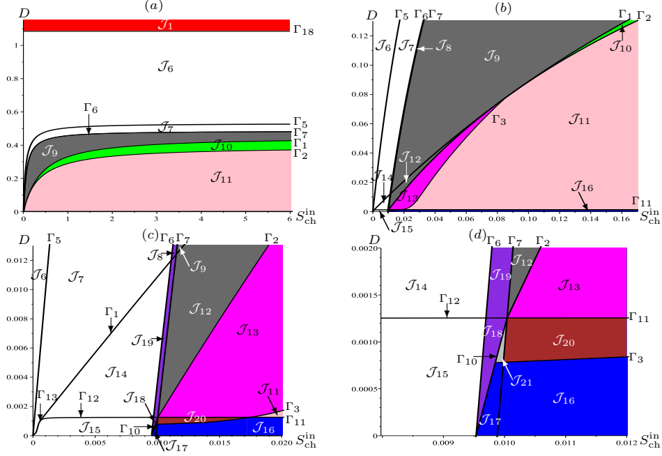
FIGURE 2. Operating diagram in the plane (S_{\text{ch}}^{\text{in}}, D) , when S_{\text{ph}}^{\text{in}} = 0 , S_{\text{H}_2}^{\text{in}} = 2.67 \times 10^{-5} and k_{\text{dec},i} = 0 . Magnifications (b) for D \in [0, 0.13] showing the regions \mathcal{J}_i , i = 12, \dots, 16 , (c) for D \in [0, 0.013] showing the regions \mathcal{J}_8 and \mathcal{J}_i , i = 17, \dots, 20 , (d) for D \in [0, 0.002] showing the region \mathcal{J}_{21} .
