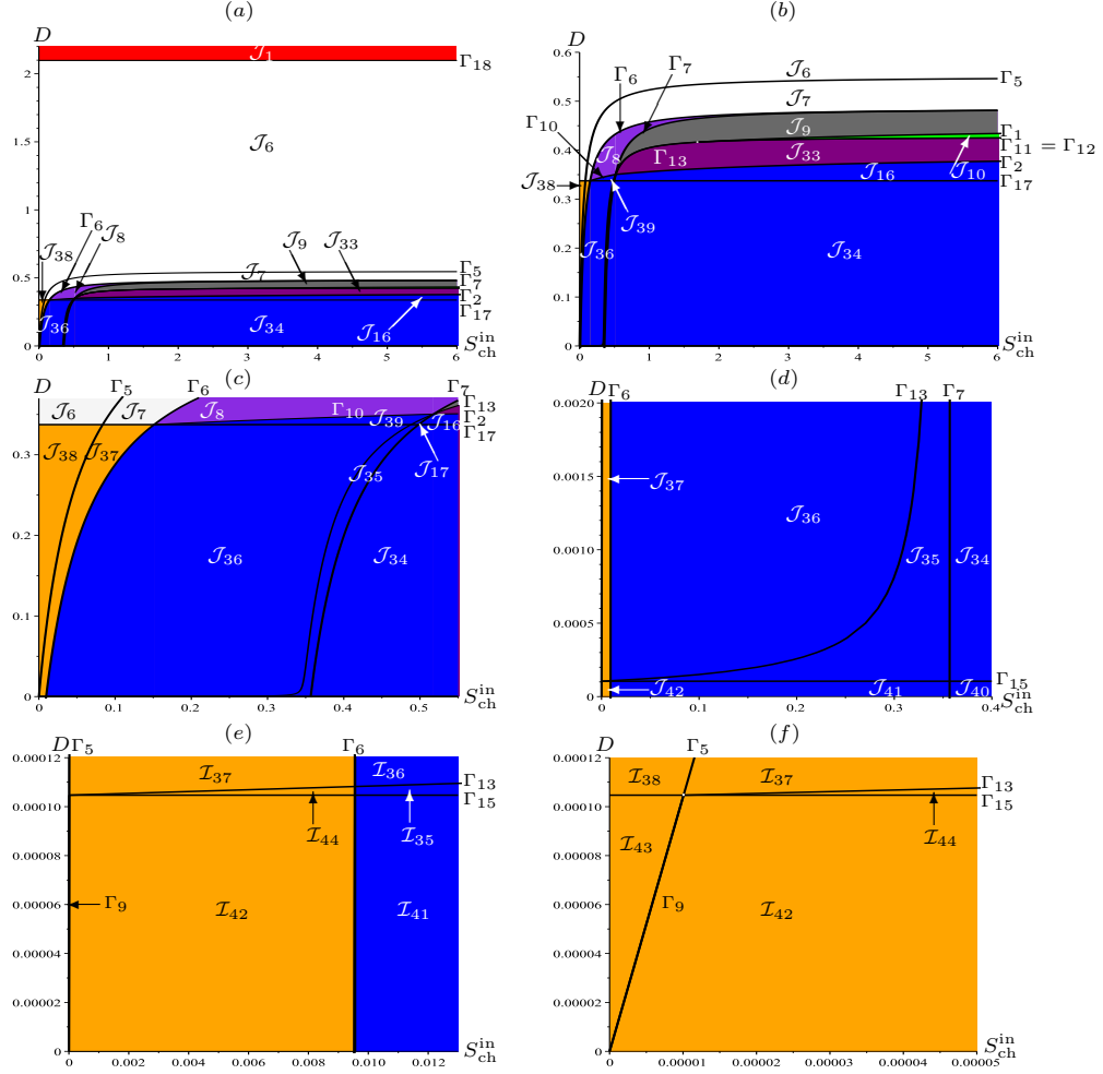
FIGURE 6. Operating diagram in the plane (S_{\text{ch}}^{\text{in}}, D) , when S_{\text{ph}}^{\text{in}} = 1 , S_{\text{H}_2}^{\text{in}} = 2.67 \times 10^{-2} and k_{\text{dec},i} = 0 . Magnifications (b) for D \in [0, 0.6] showing the regions \mathcal{J}_{10} and \mathcal{J}_{39} , (c) for D \in [0, 0.37] showing the regions \mathcal{J}_{17} , \mathcal{J}_{35} and \mathcal{J}_{37} , (d) for D \in [0, 0.002] showing the regions \mathcal{J}_{40} , \mathcal{J}_{41} and \mathcal{J}_{42} , (e) for D \in [0, 0.00012] showing the region \mathcal{J}_{44} , (f) for S_{\text{ch}}^{\text{in}} \in [0, 0.00005] showing the region \mathcal{J}_{43} .
