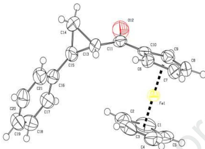
Fig. 3. ORTEP structure of Ferrocenyl 2-Phenylcyclopropyl Ketone
