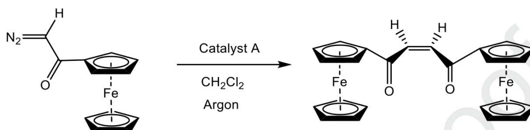
Scheme 3. Dimerization of diazoacetylferrocene catalyzed by ruthenium porphyrin
