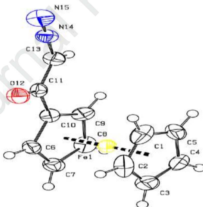
Fig. 2. ORTEP structure of diazoacetylferrocene
