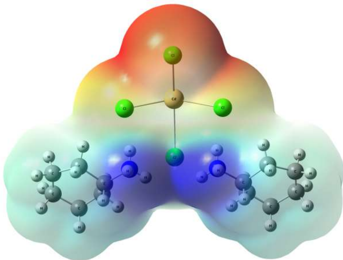
Fig. 8. Molecular electrostatic potential surface (MEPs) of (C_6H_{14}N)_2[CdCl_4] .
