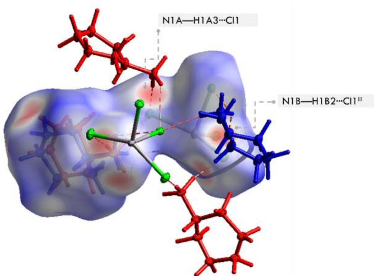
Fig. 3. 3D Hirshfeld surfaces mapped with d_{norm} in the range [-0.806 to 1.173] of (C_6H_{14}N)_2[CdCl_4] , red dotted lines represent hydrogen bonds. (iii) x, -y, z-1/2 .
