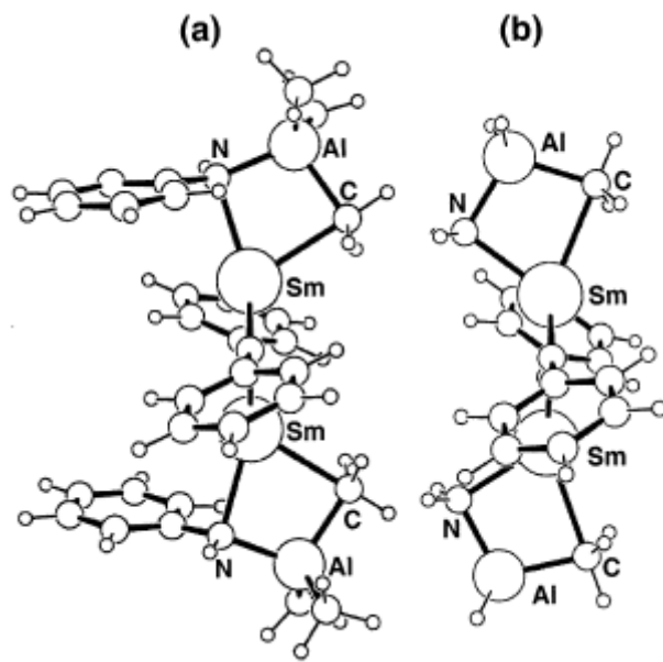
Figure 5. Views of the fully optimized [(\mu\text{-PhN})\text{Sm}(\mu\text{-NHR})(\mu\text{-Me})\text{AlR}'_2]_2 models.
