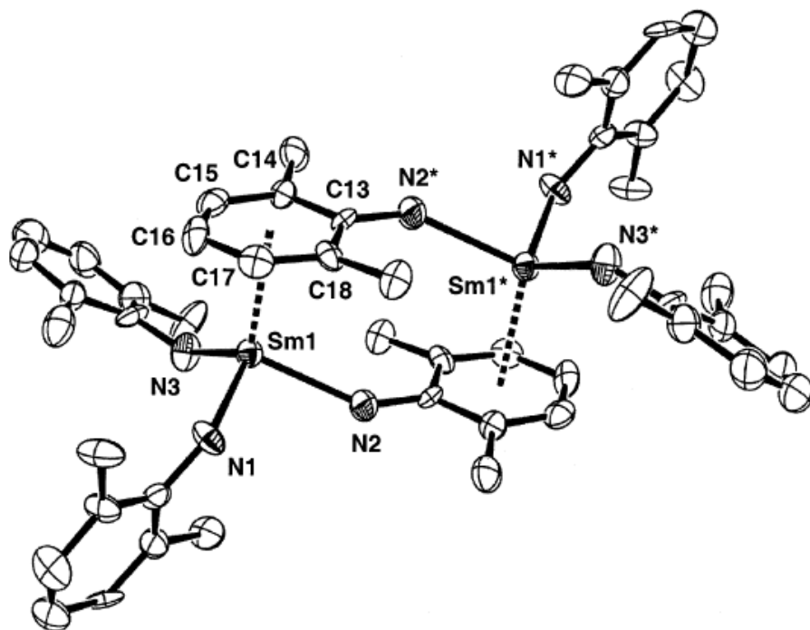
Figure 1. ORTEP view of [\text{Sm}(\mu\text{-NHC}_6\text{H}_3^i\text{Pr}_2\text{-2,6})(\text{NHC}_6\text{H}_3^i\text{Pr}_2\text{-2,6})_2] ( 1 ) drawn with 30% probability ellipsoids. Isopropyl methyl groups have been omitted for clarity.
