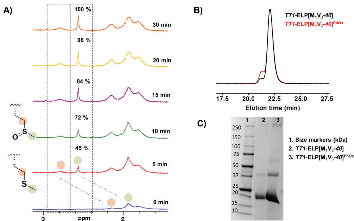
Figure 3. (A) Stacked 1 H NMR spectra of TT1-ELP[M 1 V 3 -40] after photoirradiation during 5, 10, 15, 20, and 30 minutes (D 2 O, room temperature, 200 MHz). (B) SEC chromatograms in DMSO of TT1-ELP[M 1 V 3 -40] before (black curve, RI detection) and after photoirradiation (red curve, RI detection). (C) SDS-PAGE analysis (coomassie blue stain).
