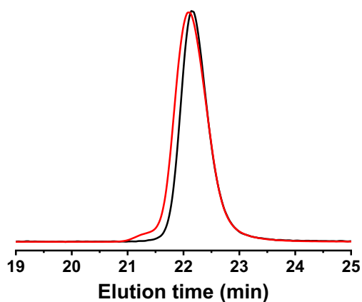
Figure S7. Size exclusion chromatograms (RI detection) in DMSO of \text{ELP}[\text{M}_1\text{V}_3\text{-40}] (black curve) and \text{ELP}[\text{M}(\text{O})_1\text{V}_3\text{-40}] (red curve).
