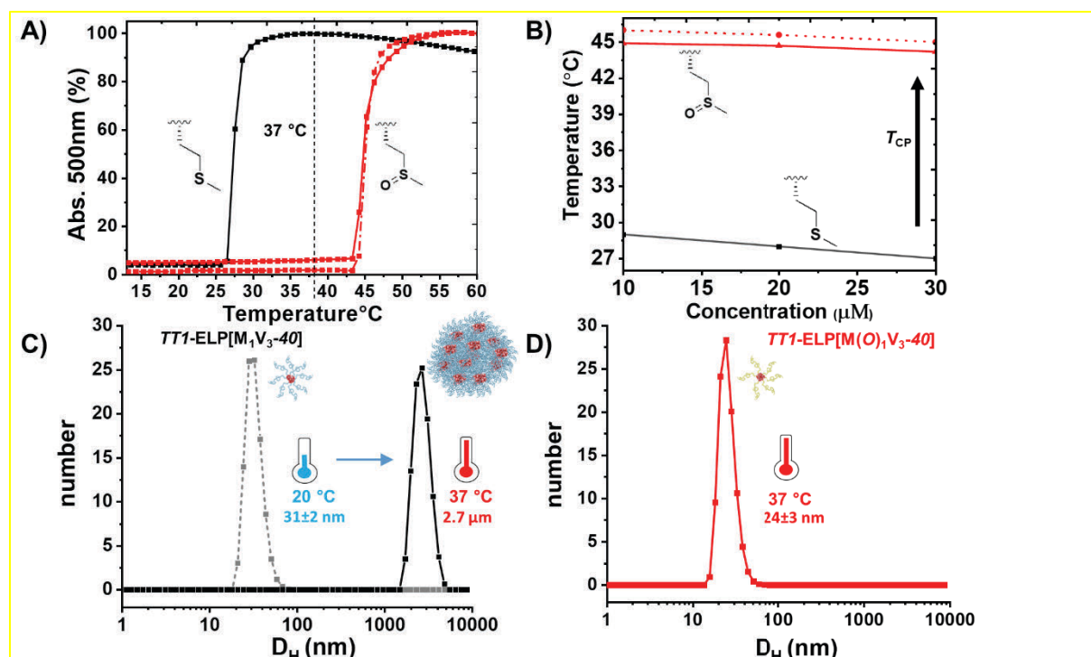
Figure 4. A) Normalized relative absorbance at 500 nm of 30 μM solution of TT1-ELP[M 1 V 3 -40] (black trace), TT1-ELP[M 1 V 3 -40] PhOx (red trace) and TT1-ELPM(O) 1 V 3 -40] (red dots) conjugates in PBS as a function of temperature. B) Transition temperature ( T_{CP} ) versus molar concentration of TT1-ELP[M 1 V 3 -40] (black), TT1-ELP[M 1 V 3 -40] PhOx (red) and TT1-ELP[M(O) 1 V 3 -40] (red dots). C) Size distribution (in number) of TT1-ELP[M 1 V 3 -40] at 20 °C and 37 °C (30 μM concentration in PBS). D) Size distribution (in number) of TT1-ELPM(O) 1 V 3 -40] at 37 °C (30 μM concentration in PBS).
