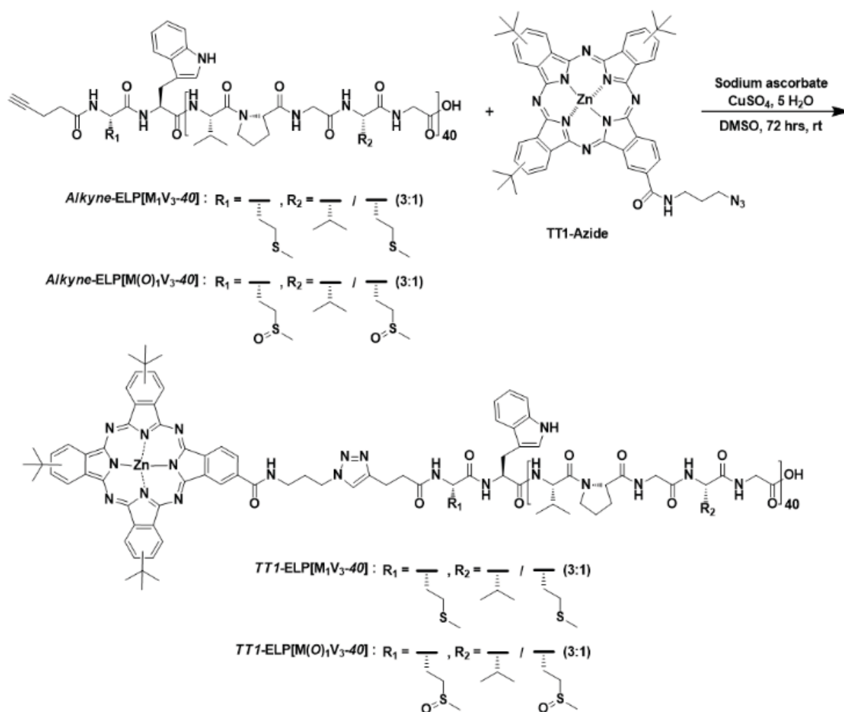
Scheme 1. Synthetic scheme to access TT1 -ELP[M 1 V 3 -40] and the reference compound TT1 -ELP[M(O) 1 V 3 -40].
