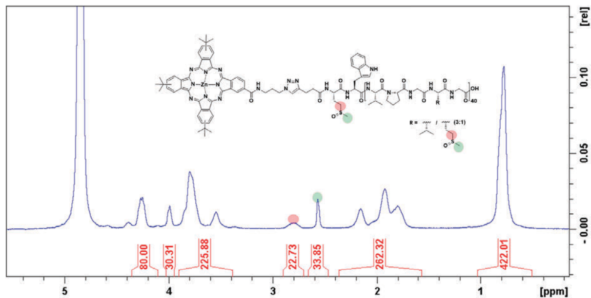
Figure S9. ^1\text{H} NMR spectrum of TT1 -ELP[M(O) 1 V 3 -40] in D 2 O at 5 °C.
