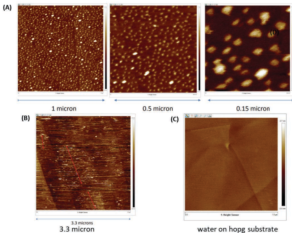
Figure S12. Temperature-Controlled High-Speed AFM (liquid) images of TTI-ELP [ M_1V_3-40 ] on HOPG substrate (A) at 15 ^{\circ}\text{C} , (B) at 50 ^{\circ}\text{C} in PBS and (C) pure water on HOPG substrate.
