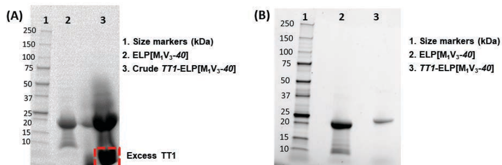
Figure S4. SDS-PAGE analysis of TT1 -ELP[M 1 V 3 -40] (A) before and (B) after purification.
