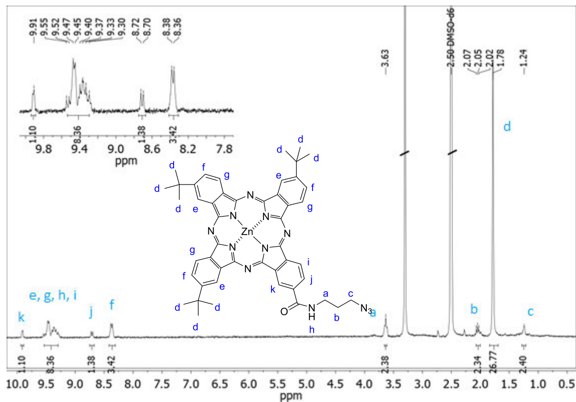
Figure S1. ^1\text{H} NMR spectrum of TT1-amide-C3-azide (1) ( \text{DMSO-d}_6 ).
