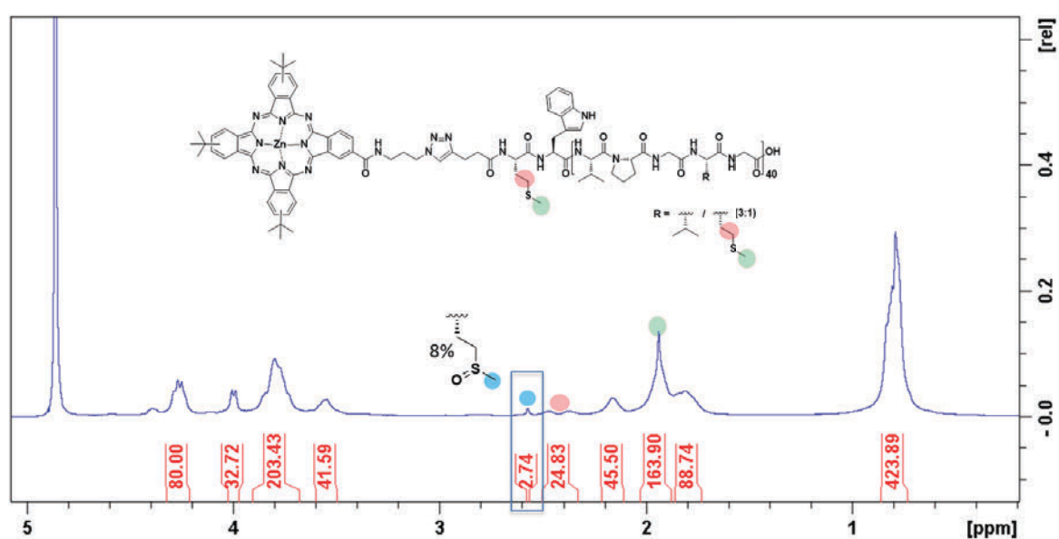
Figure S5. 1 H NMR spectrum of TT1 -ELP[M 1 V 3 -40] in D 2 O at 5 °C.
