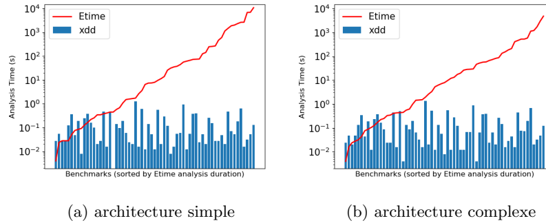
Figure 2: Temps d'analyse de XDD vs. Etime (exhaustif).
