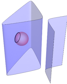
FIGURE 7. The curve X'_1 .
