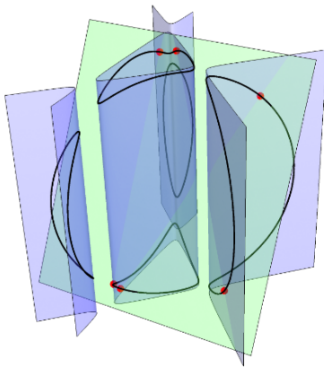
FIGURE 1. A real space curve of degree 6 with a totally real hyperplane section.
