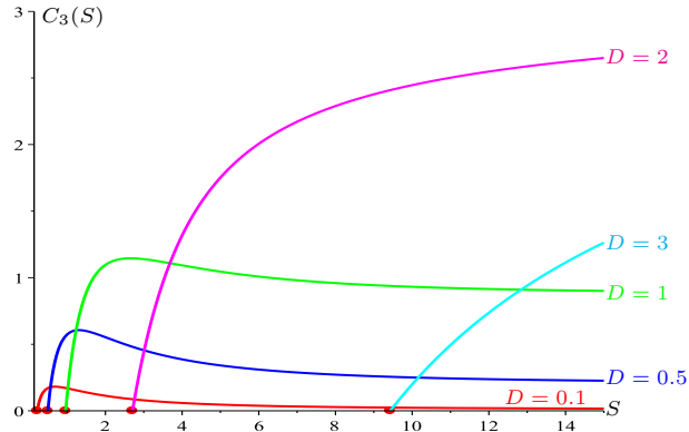
FIGURE 3. Curves of the function C_3(S) for different values of D when S > \max(\lambda_1(D), \bar{\lambda}_2(D)) .
