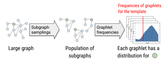
Figure 5. Computing pipeline for a graphlet similarity measure between a template and a large graph. The green node is a specific node of the large graph.
