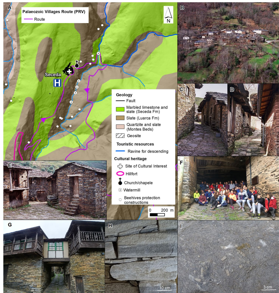
Fig. 7 Seceda Devonian Village. A Geological map of the surroundings after Villar-Alonso et al. (2018), showing the nearby tourism resources, cultural heritage, and geosites. B Overview of the village walled using Devonian marbled limestone and shale. C–G Traditional buildings and pavements. H Marbled limestone from a traditional dwelling. I Crinoids
