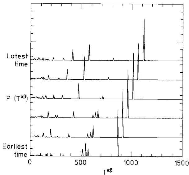
Fig. 1. Distribution of the elements of the matrix T^{\alpha\beta} in the OPM for a population of M = 1000 individuals. The distribution is shown at six times for the same population. There is a period of 50 generations between each successive pair of curves; therefore the peaks move a distance 50 to the right each time. Peaks fluctuate in size and eventually disappear.
