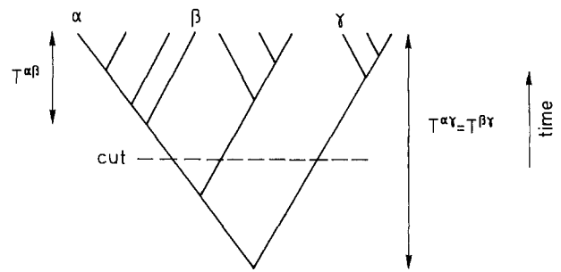
Fig. 2. Schematic representation of the genealogical tree in the OPM showing ultrametric property of the branching times T^{\alpha\beta} , T^{\alpha\gamma} , T^{\beta\gamma} . Cutting the tree at an arbitrary point in the past divides the population into families.
