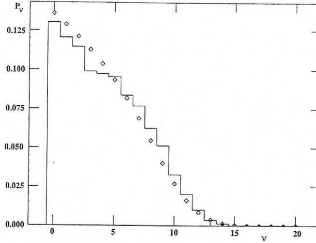
Figure 4. Histograms of the Hamming distance \nu for N=20 , M=200 : (a) \lambda=0.6 ; (b) \lambda=1.0 ; (c) \lambda=1.5 . Diamonds: equation (42). Averages over 10 000 generations.
