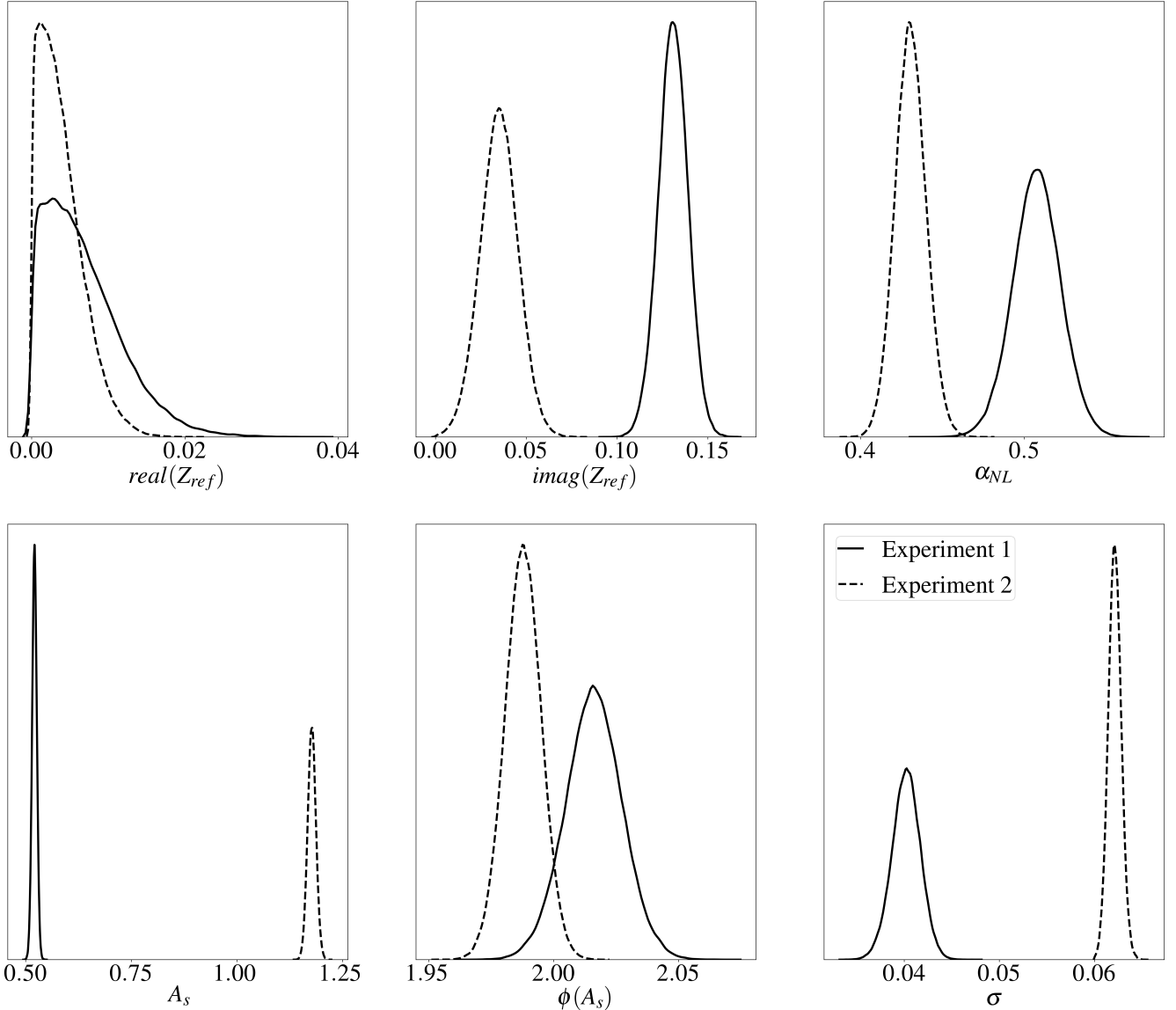
Figure 12: Posterior probability density functions of the educed parameters, in Experiments 1 (140 dB) and 2 (147 dB).
