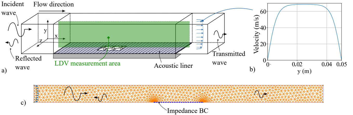
Figure 1: a) Schematics of the B2A aeroacoustic bench and LDV measurement area. b) Flow profile used in the simulations at Mach 0.2. c) Schematics of the mesh used throughout this study.
