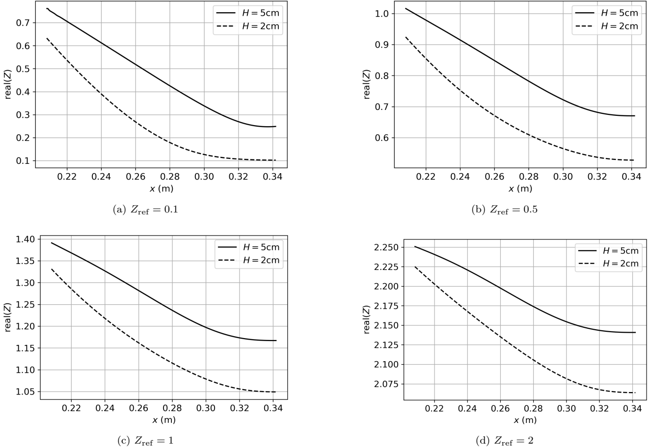
Figure 7: Converged spatially-varying impedances, without flow, for different duct heights H . Incident SPL = 140 dB, f = 1\text{ kHz} , \alpha_{\text{NL}} = 1.2 .
