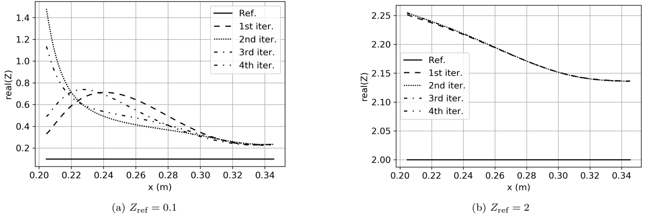
Figure 4: Spatially-varying impedance at the first iterations. Incident SPL = 140 dB, \alpha_{\text{NL}} = 1.2 , f = 1 kHz. Converged impedance values were given in Fig. 2.
