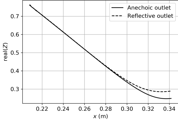
(a) Converged impedances. Z_{\text{ref}} = 0.1
