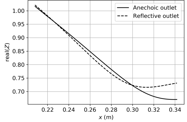
(b) Converged impedances. Z_{\text{ref}} = 0.5
