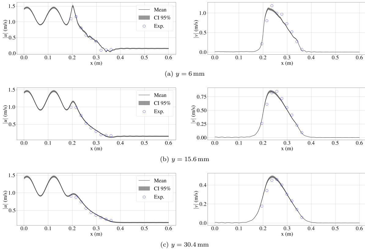
Figure 15: Comparison between experimental and inferred velocity fields in Experiment 2, at different heights in the B2A. Incident SPL is approximately 147 dB, and the incident wave comes from the left.
