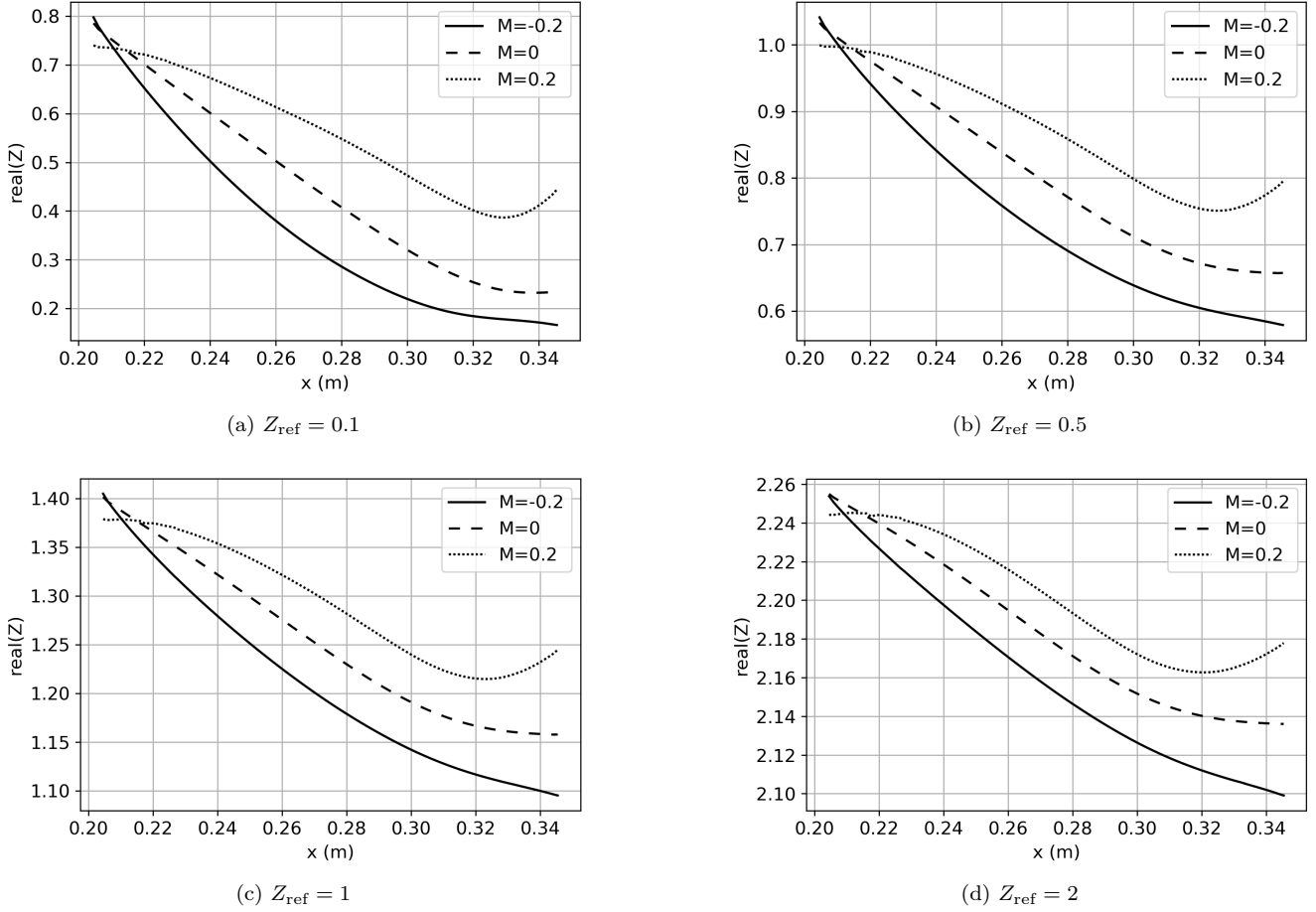
Figure 6: Converged spatially-varying impedances at different Mach numbers and different reference (constant) impedances. The incident wave comes from the left, with incident SPL = 140 dB, f = 1 kHz. For all cases, the nonlinear factor is \alpha_{\text{NL}} = 1.2 in Eq. 5.
