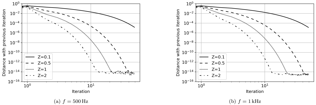
Figure 3: Convergence analysis of the spatially-varying impedance, for different reference impedances without flow, at different frequencies. Incident SPL = 140 dB. \alpha_{NL} = 1.2 .
