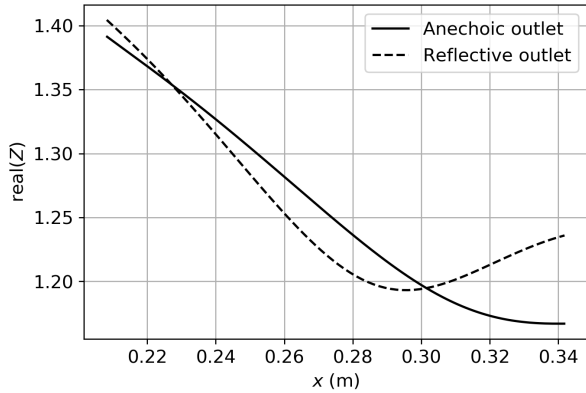
(c) Converged impedances. Z_{\text{ref}} = 1
