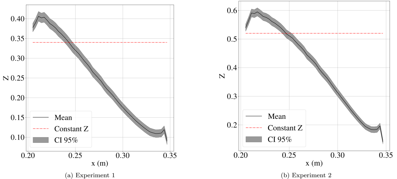
Figure 13: Educued spatially-varying impedance and 95% confidence intervals. The dashed horizontal line corresponds to the value identified when the impedance is assumed constant spatially.
