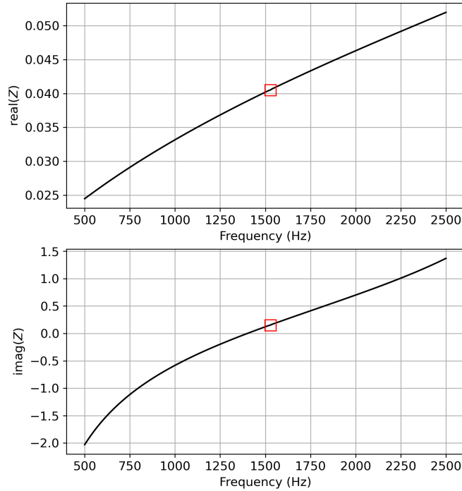
Figure 10: Reference impedance values of the IFAR liner sample as a function of the frequency, evaluated with a rigid equivalent fluid assumption and a transfer matrix method. The red symbols indicate f = 1528\text{ Hz} . Z_{\text{ref}}(f = 1528\text{ Hz}) \approx 0.04 + 0.21j .
