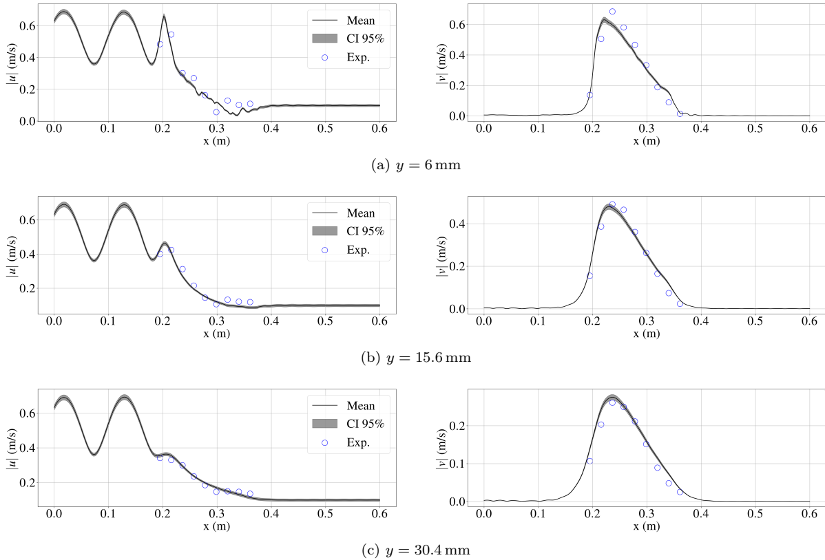
Figure 14: Comparison between experimental and inferred velocity fields in Experiment 1, at different heights in the B2A. Incident SPL is approximately 140 dB, and the incident wave comes from the left.
