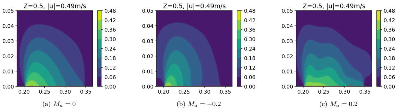
Figure 5: Converged |v| fields in the x-y plane at different Mach numbers. The reference impedance is Z_{\text{ref}} = 0.5 , and the frequency is f = 1 kHz, at an incident wave coming from the left with an incident SPL of 140 dB. This corresponds to an incident particle velocity of \approx 0.49 m/s. The dashed red line represents the liner position in the duct. M_a is the average Mach number.
