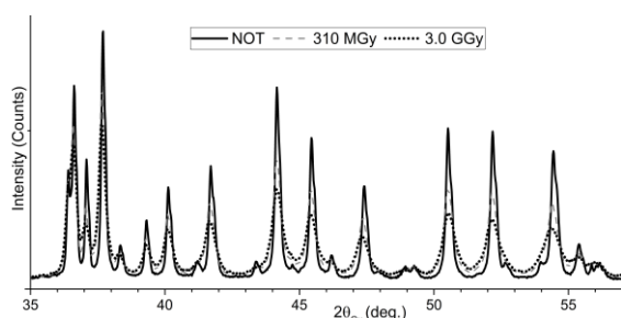
Figure 5. X-Ray diffraction pattern of gibbsite \text{Al(OH)}_3 : before irradiation and after electron irradiation at two doses (310 MGy, 3 GGy).
