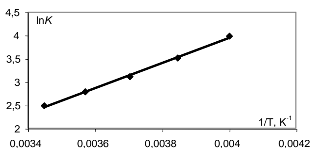
Figure 3. Temperature dependence of lnK for the interaction between Cp*Fe(dppe)H and TFE in CH 2 Cl 2 . [Fe] = 0.13 M; [TFE] = 0.01 M.
