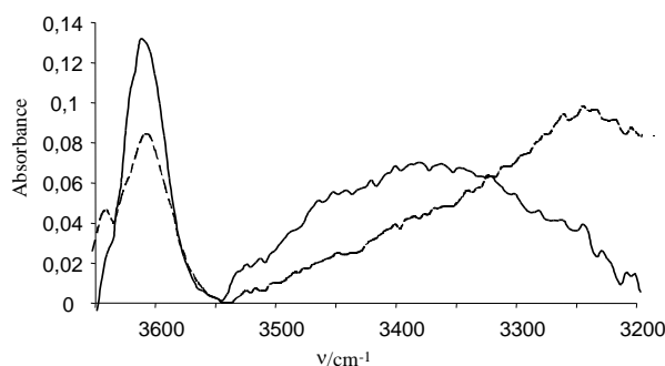
Figure 2. IR spectra in the \nu(\text{R}_F\text{O-H}) stretching region showing the interaction between \text{Cp}^*\text{Fe}(\text{dppe})\text{H} and MFE or TFE in \text{CH}_2\text{Cl}_2 . Solid line: [\text{Fe}] = 0.15 \text{ M} ; [\text{MFE}] = 0.015 \text{ M} . Dashed line: [\text{Fe}] = 0.13 \text{ M} ; [\text{TFE}] = 0.01 \text{ M} .
