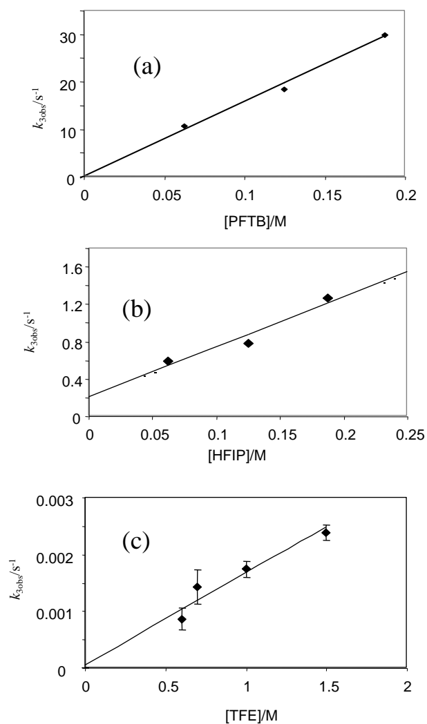
Figure 7. Pseudo-1 st order rate constants for the first step of the proton transfer from HA to \text{Cp}^*\text{Fe}(\text{dppe})\text{H} [ k_{3\text{obs}} ; HA = PFTB (a), HFIP (b), TFE (c)].
