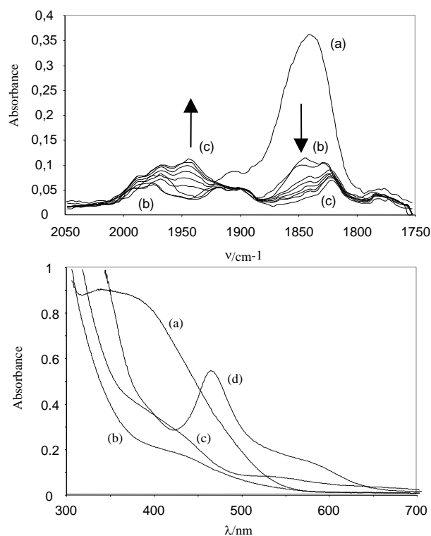
Figure 1. Spectral changes (IR, above; UV-visible, below) observed for the protonation of \text{Cp}^*\text{Fe}(\text{dppe})\text{H} by \text{HBF}_4 in \text{CH}_2\text{Cl}_2 . (a) Before addition of \text{HBF}_4 ( T = 200\text{K} ); (b) after addition of \text{HBF}_4 ( T = 200\text{K} ); (c) T = 290 \text{ K} (after a few minutes); (d) T = 290 , after several hours. [\text{Fe}] = 0.03 \text{ M} (IR); 0.01 \text{ M} (UV-visible); \text{HBF}_4/\text{Fe} = 1 .
