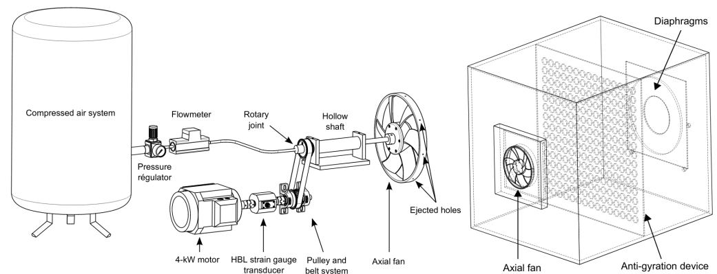
Figure 3. Experimental setup: (a) the fan drive system, (b) ISO – 5801 test bench (dimensions 1.3 \times 1.3 \text{ m} \times 1.8 \text{ m} ).
