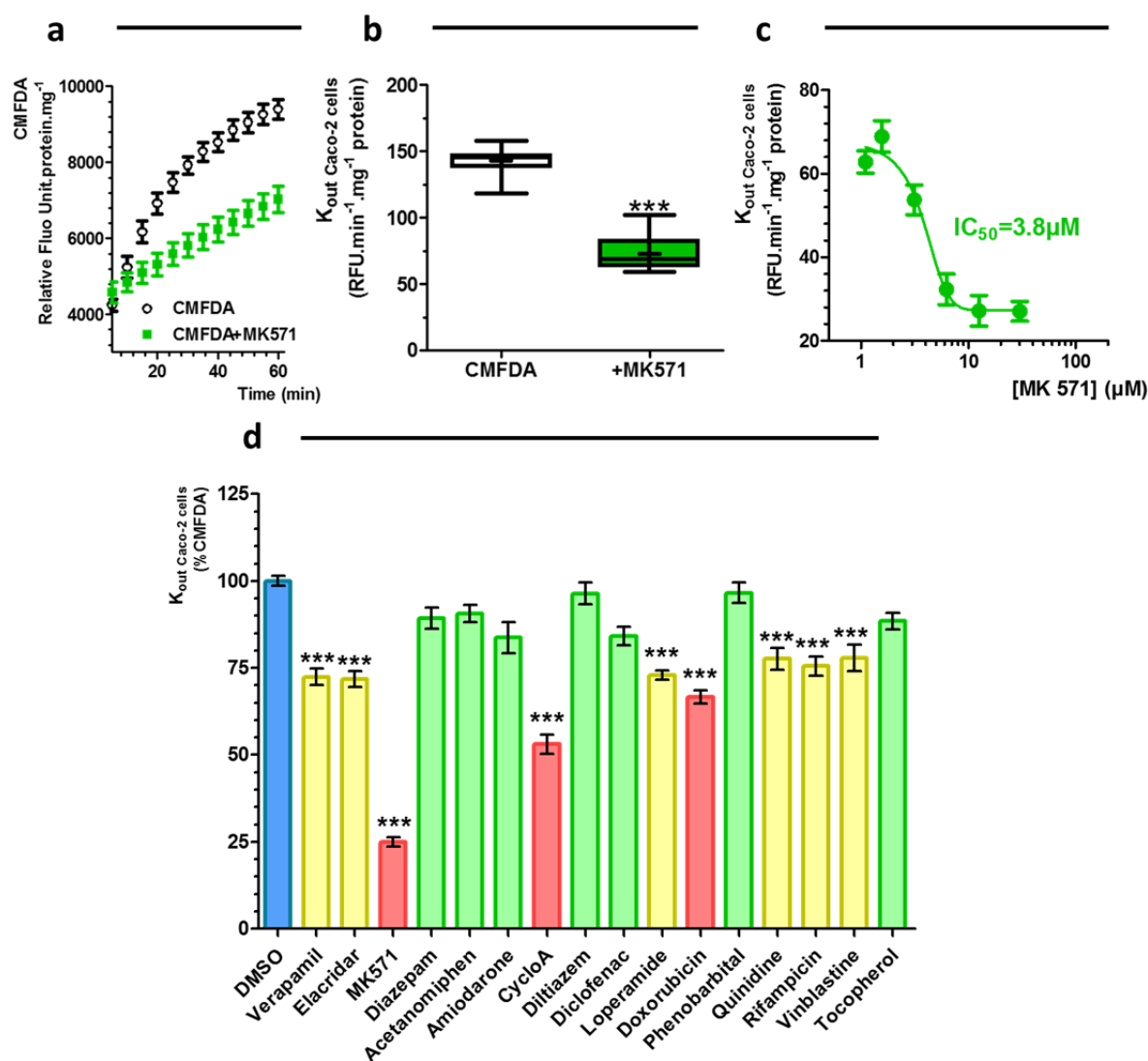
Figure 5. (a) Excretion of CMFDA after incubation of cell Caco-2 monolayers in absence or in presence of 50 \mu\text{M} MK571, (mean \pm s.e.m, n = 12 ). (b) Rate of excretion of CMFDA after an incubation of cell Caco-2 monolayers in absence or in presence of 50 \mu\text{M} MK571 box-and-whisker diagram, whiskers: min to max, mean: cross, n = 12 , *** p < 0.001 ). (c) Concentration-dependent effects of MK571 on CMFDA excretion from Caco-2 cells (mean \pm s.e.m, n = 12 ). (d) Effect of drugs on Rate of excretion of CMFDA (mean \pm s.e.m, n = 12 –54, *** p < 0.001 ).
