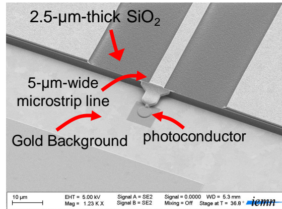
Figure 21: Optical cavity LT-GaAs photoconductor
