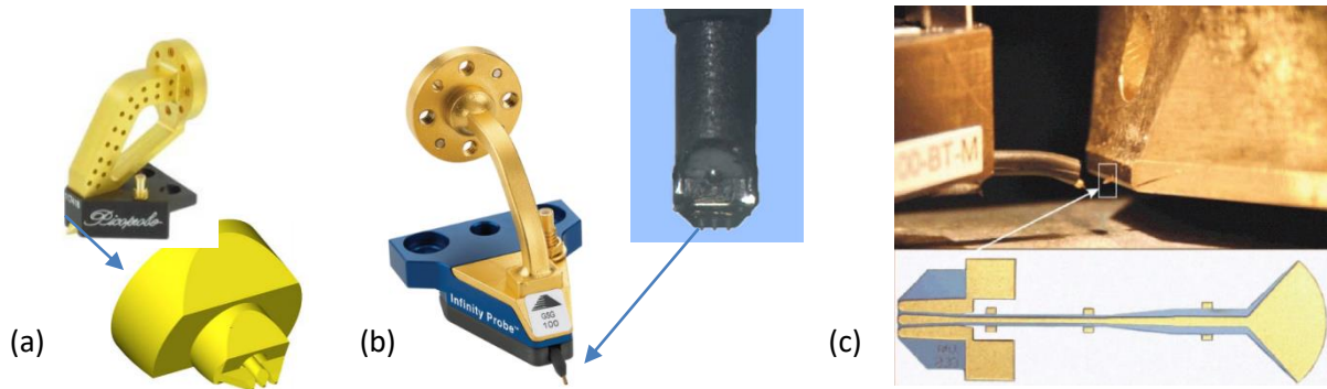
Figure 38: Different probes technologies: GGB probes [87] (a), Infinity-micro-coax (b), up to 500 GHz[86] and micromachined probes (c) [90].
