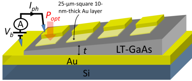
Figure 19: Experimental set-up aimed at photoresponse measurement
