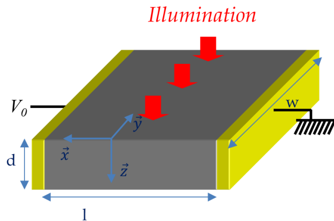
Figure 2: Photomixing in a photoconductor
