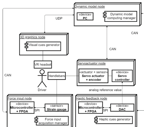
Figure 4: Deployment diagram of our POC system.
