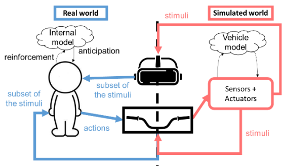
Figure 2: Schematic representation of the interactions between the driver and our POC system.
