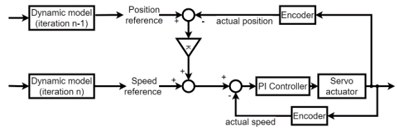
Figure 5: Block diagram representation of the servo actuator's position-speed control.
