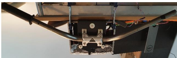
Figure 3: Haptic feedback motorcycle handlebars used in our POC system.
