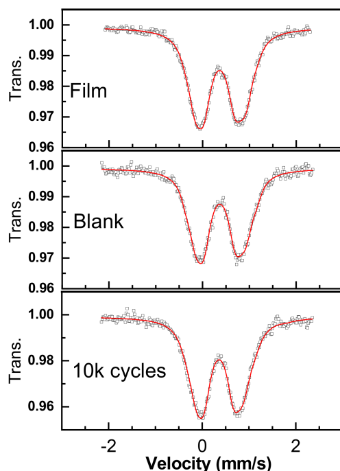
Figure 7. Room temperature Mössbauer spectra for non-cycled FWO-600 electrode (“Film”), non-cycled but soaked in electrolyte (“Blank”) and cycled electrode after 10,000 cycles at 20 \text{ mV s}^{-1} (“10k cycles”).
