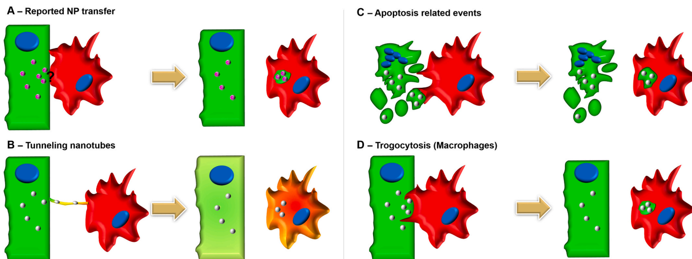
Scheme 1. Illustrations of the reported NP transfer and known Cell-Cell transfer mechanisms.
