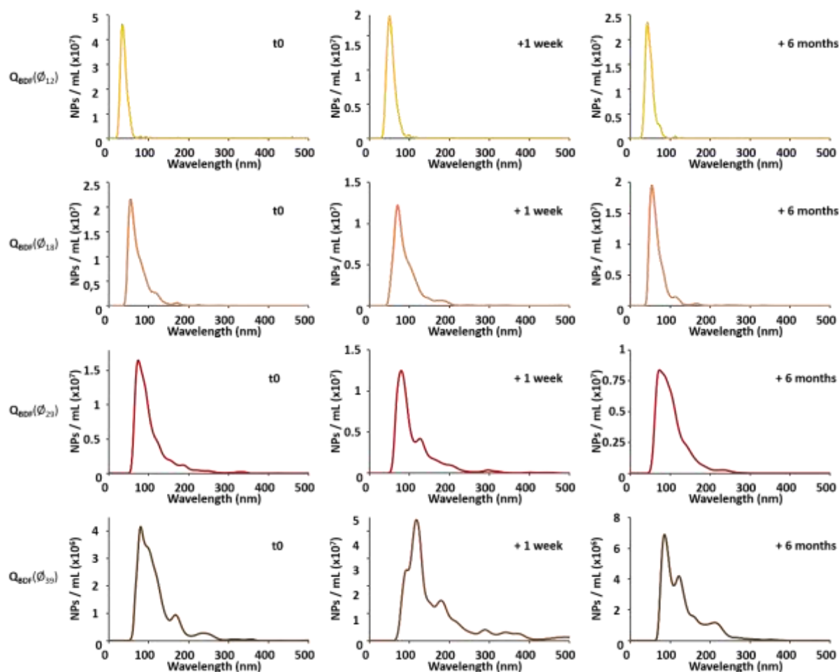
Supplementary Figure S6: Distributions of hydrodynamic diameters of Q_{BDF} FONs in water as measured using NTA. Diameters were measured within 48h of FONs preparation (Left), one week later (Middle) or 6 months later (Right)
