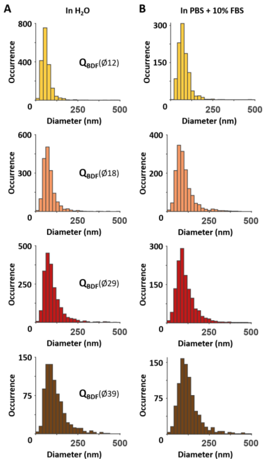
Supplementary Figure S7. Size distributions of Q_{BDF} FONs determined by Single Particle Tracking in A mQ grade water and B PBS supplemented with 10% FBS. Analysis was performed on 3 to 5 fields of view per preparation.
