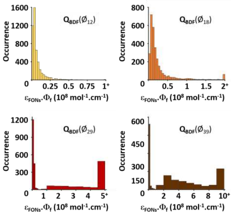
Supplementary Figure S3. Distribution of FONs brightness in relation with their size distribution. For comparison, the brightness of the molecular form in low-medium polarity organic solvent is 2 \cdot 10^4 \text{ M}^{-1} \text{ cm}^{-1} .
