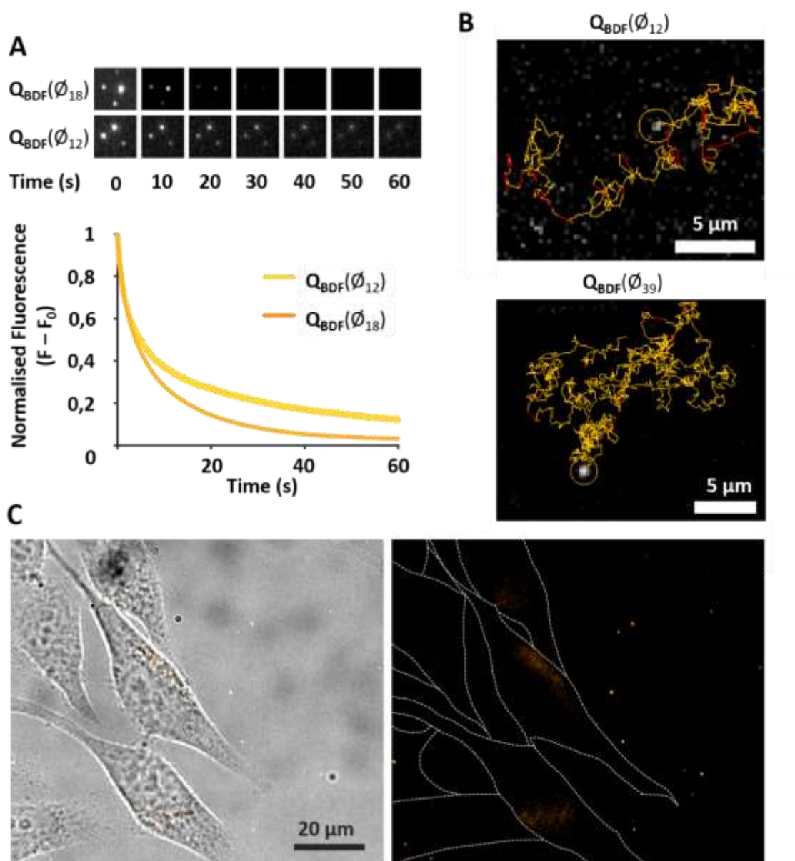
Figure 2. A (Top) Example regions of interest and (Bottom) average trace of Q_{\text{BDF}} FONs intensity decaying with time. B Example trajectory of a single Q_{\text{BDF}}(\varnothing_{12}) (Top) and Q_{\text{BDF}}(\varnothing_{39}) (Bottom) FON in water. C Example fluorescence image of Q_{\text{BDF}}(\varnothing_{18}) FONs incubated for 24h with HeLa cells; (Left) overlaid with a bright field image. (Right) with cell contours traced for clarity.
