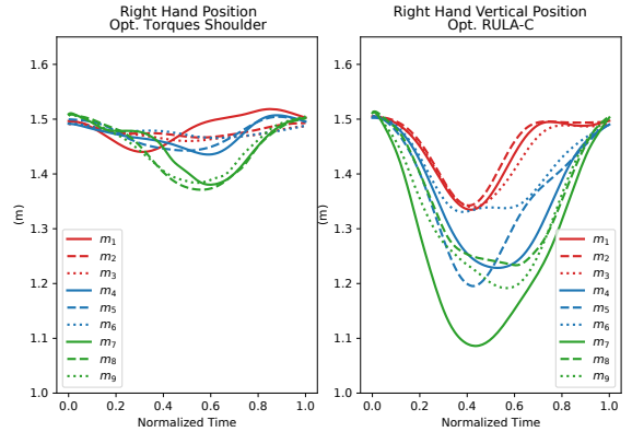
Fig. 4: Optimized hand trajectories w.r.t. torques shoulder and RULA-C scores for the morphologies m_i | i \in [1 \dots 9] in Tab. II in experiment 1. Tall in red, medium in blue, and short in green.
