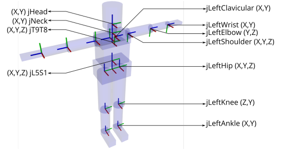
Fig. 2: Digital Human Model (DHM) joints description. The axes are X=Red, Y=Green, Z=Blue.
