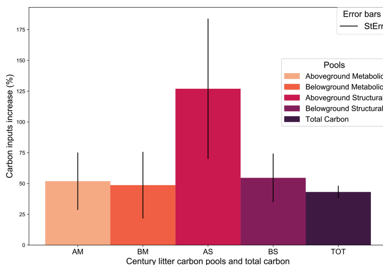
Figure 6. Site average percentage change of carbon inputs needed to reach the 4p1000 (TOT), separated into the four litter input pools. AM: aboveground metabolic; BM: belowground metabolic; AS: aboveground structural; BS: belowground structural; TOT: total litter inputs. Error bars indicate the standard error. N.B: total change of carbon inputs (TOT) was calculated as the percentage change between the total amount of carbon inputs before and after the 4p1000 optimization, averaged across all sites.
