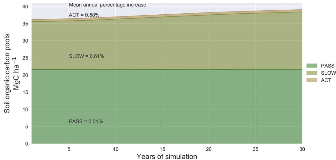
Figure 7. Sites average soil organic carbon pools (ACT: active; SLOW: slow; PASS: passive) evolution ( \text{MgC ha}^{-1} ) over the 30 years of simulation to reach the 4p1000 target. In the graph the mean percentage increase is given for each SOC pool.
