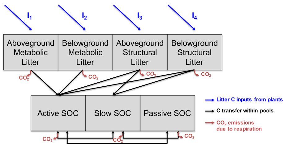
Figure 3. Representation of litter and soil organic carbon (SOC) pools in Century. The model takes as input litter carbon from plants (aboveground metabolic ( I_1 ), belowground metabolic ( I_2 ), aboveground structural ( I_3 ) and belowground structural ( I_4 )). A certain fraction of carbon can be transferred from one pool to another, and each time a transfer occurs, part of this carbon is respired and leaves the system to the atmosphere as \text{CO}_2 . The SOC active pool receives carbon from each litter pool, while only the structural material is transferred to the SOC slow pool. Litter material never goes directly to the SOC passive pool while the three SOC pools exchange C within each other.
