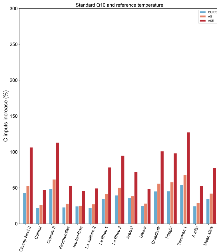
Figure C1. Temperature sensitivity analysis of carbon input change (%) to reach the 4p1000 objective, using Century default Q_{10} and reference temperature parameters. CURR: business-as-usual simulation; AS1: RCP2.6 scenario of +1 °C temperature increase; AS5: RCP8.5 scenario of +5 °C temperature change.
