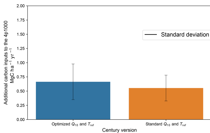
Figure C2. Effect of the optimization of the Q_{10} and reference temperature ( T_{\text{ref}} ) parameters on the additional carbon inputs to reach the 4p1000 predicted by Century (mean \pm standard deviation).
