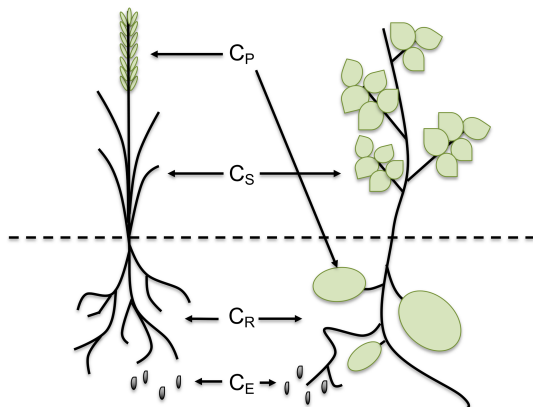
Figure 2. Adapted from Bolinder et al. (2007). Representation of the distribution of carbon in the different parts of the plant: C_P represents the carbon in the harvested product (grain, forage, tuber), C_S is the carbon in the aboveground residue (straw, stover, chaff), C_R is the carbon present in roots and C_E represents all the extra-root carbon (including all root-derived materials not usually recovered in the root fraction).
