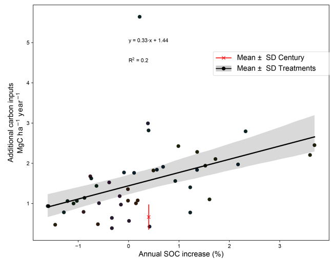
Figure 5. Correlation between additional carbon inputs ( \text{MgC ha}^{-1} per year) and annual SOC stock increase (%) in the carbon input treatments and mean \pm standard deviation of the additional carbon inputs to reach the 0.4 % target in Century.
