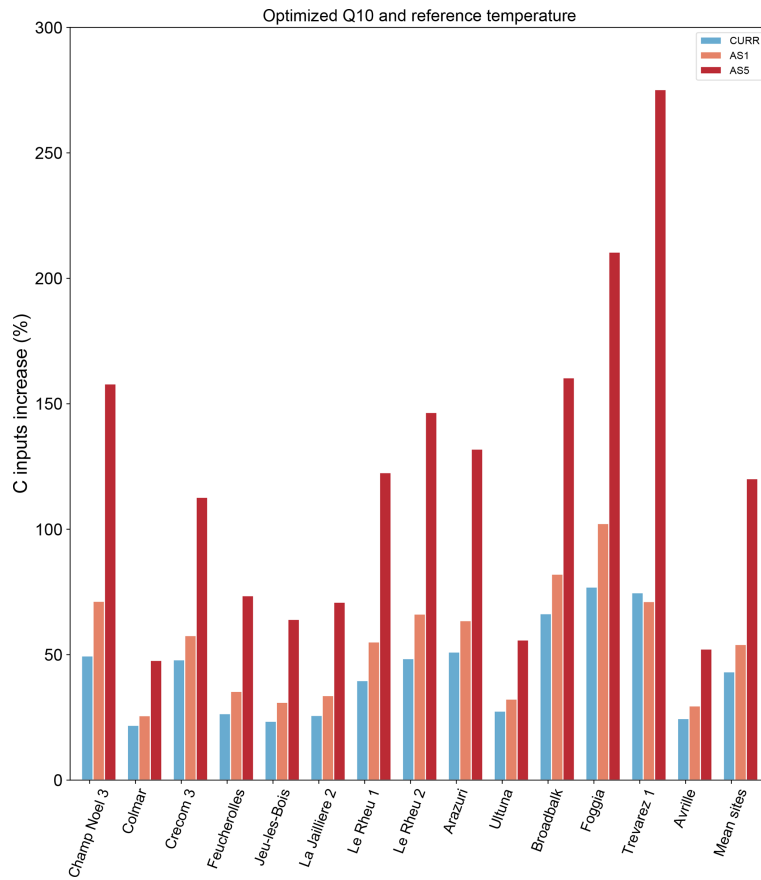
Figure 10. Temperature sensitivity analysis of carbon input increase (%) to reach the 4p1000 objective. CURR: business-as-usual simulation; AS1: RCP2.6 scenario of +1 °C temperature increase; AS5: RCP8.5 scenario of +5 °C temperature change.
