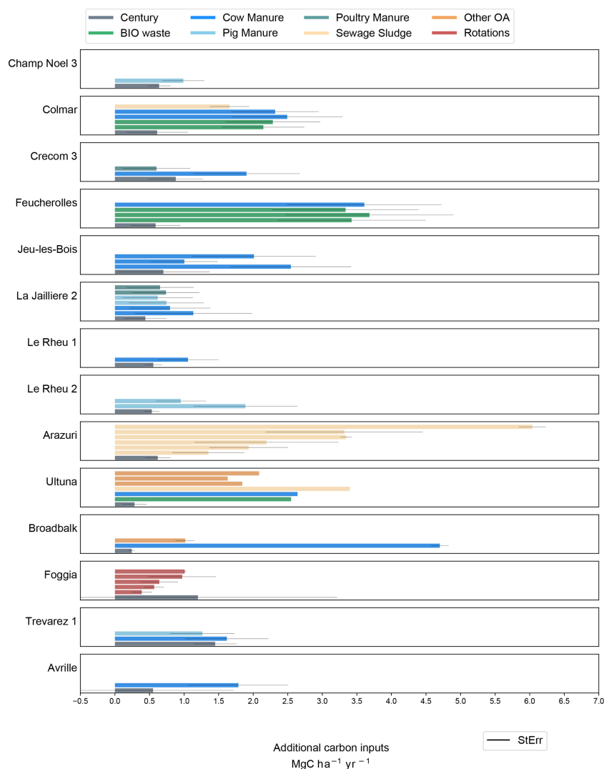
Figure 9. Additional modeled carbon inputs ( \text{MgC ha}^{-1} \text{yr}^{-1} ) to reach the 4p1000 (grey bars) compared to additional carbon input treatments (colored bars) at each experimental site. Additional carbon inputs for field trials are calculated as the sum of organic fertilizers and the delta carbon inputs from crop yields (compared to the control plot). Additional carbon treatments are separated into different categories: BIO waste: biowaste compost, green manure, green manure and sewage sludge, and household waste; Cow manure: cow manure and farmyard manure (in Broadbalk and Ultuna), pig manure, poultry manure, sewage sludge; Rotations: different crop rotations, other organic amendments (OA): straw, sawdust, and peat (in Ultuna) and castor meal (in Broadbalk). The error bars shown are the standard errors computed with the Monte Carlo method.
