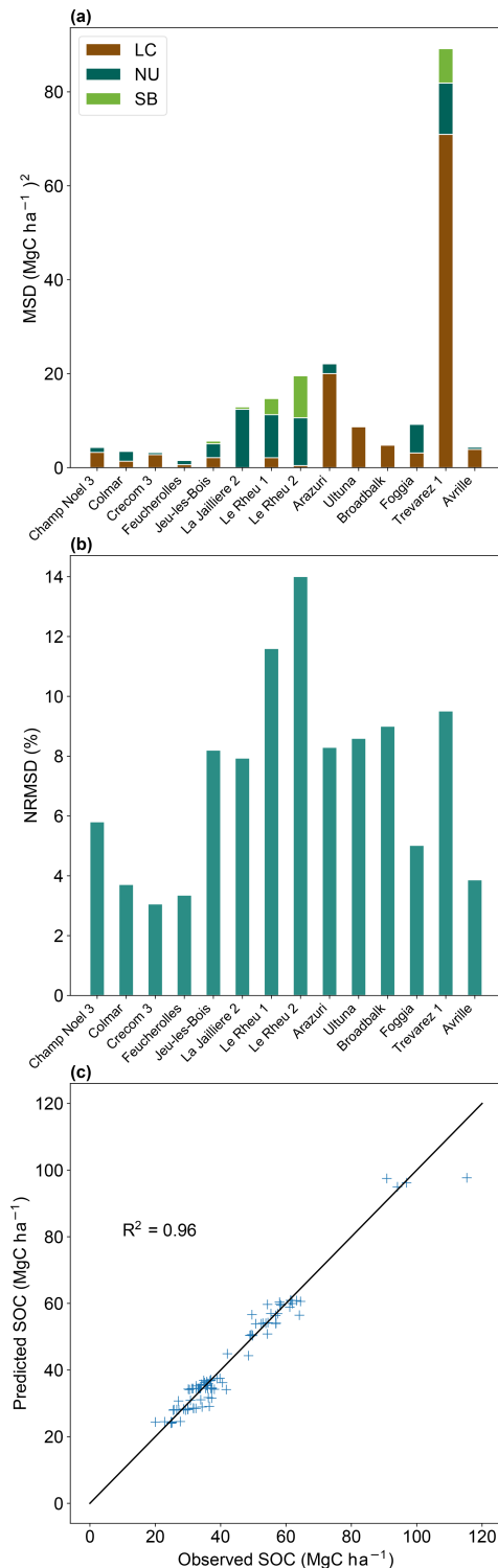
Figure 4. (a) Decomposed mean squared deviation ( \text{MgC ha}^{-1} ) 2 in control plots for all sites. LC: lack of correlation; NU: non-unity slope; SB: squared bias. (b) Normalized root squared deviation (%) in control plots for all sites. (c) Fit of predicted vs. observed SOC stocks ( \text{MgC ha}^{-1} ) to control plots for all sites ( R^2 = 0.96 ).
