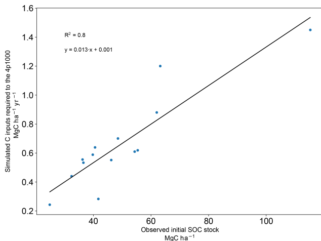
Figure 8. Correlation between initial observed SOC stocks ( \text{MgC ha}^{-1} ) and modeled carbon inputs needed to reach the 4p1000 target ( \text{MgC ha}^{-1} \text{ yr}^{-1} ). The correlation coefficient ( R^2 ) is 0.80 and the regression line is y = 0.013 \cdot x + 0.001 .
