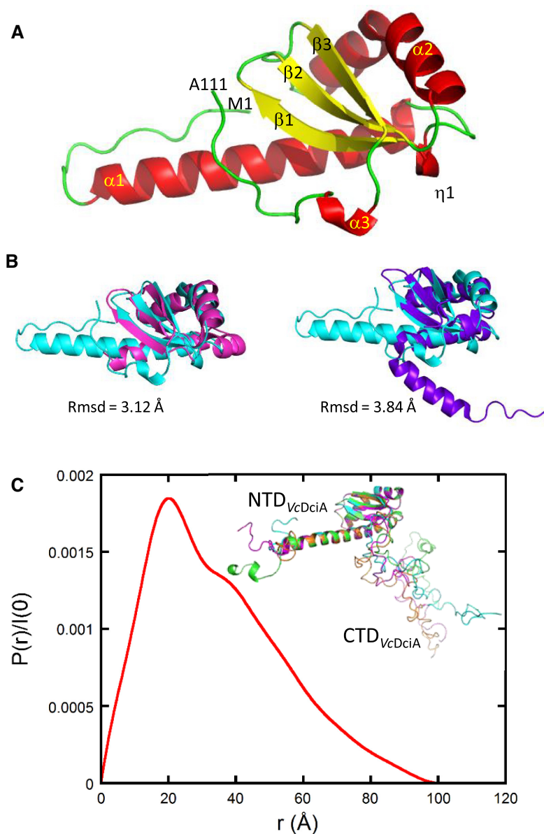
Figure 3. The NTD of VcDciA shares a common type-II KH-domain fold with the DnaB-binding domain of DnaA and with the DnaX domain V. (A) Representative structural model for VcDciA NTD (residues 1 to 111), built from NMR backbone chemical shifts. Corresponding secondary structure elements are displayed in red for \alpha -helices and yellow for \beta -strands. The regions without defined secondary structure are in green. VcDciA NTD exhibits a type-II KH-domain fold topology (51). (B) Structural superimposition between the representative NMR-based structural model of VcDciA (residues 1–111, cyan) and the homologous NTD of BsDnaA (left, PDB ID 4TPS, chain B, pink) and EcDnaX CTD (right, PDB ID 2AYA, model 1, residues 1–96, purple). (C) Distance distribution function P(r) of VcDciA resulting from SEC-SAXS analysis of the full-length protein. (Inset) Four superimposed models of the VcDciA full-length protein generated from the SAXS curve starting from the NMR model (NTD) and modeling the missing CTD residues using the program DADIMODO (see Materials and Methods and Supplementary Table S3) (28,60). The four models display random coiled VcDciA CTD.
