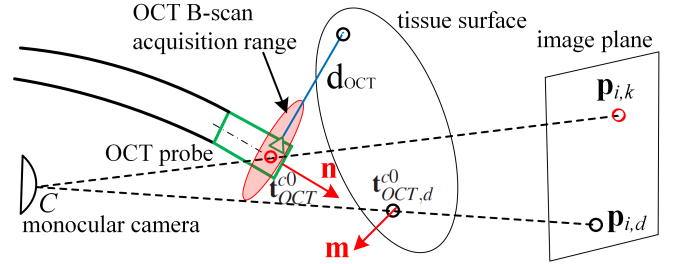
Figure 2. Illustration of the control objectives for tissue scanning. t_{OCT}^0 and t_{OCT,d}^0 are respectively the 3D position of the OCT probe and its desired position. Their corresponding image positions are p_{i,k} and p_{i,d} , respectively. \mathbf{m} is the normal direction of the surface at point t_{OCT,d}^0 . \mathbf{n} is the direction of the OCT probe. d_{OCT} is the shortest distance on the OCT imaging plane between the OCT probe and the tissue.
