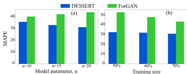
Figure 4: Model ablation w.r.t. (a) \alpha and (b) training size.
