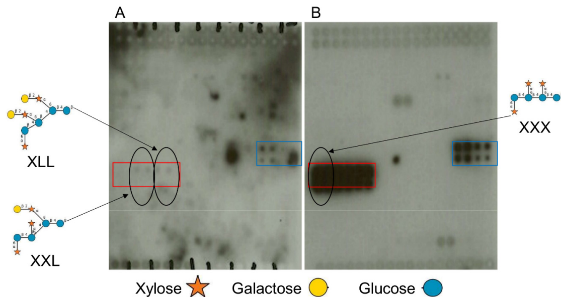
Figure 2. Plant oligosaccharide and polysaccharide interactions with F9. (A) Plant glycan arrays (approx. 2.5 cm × 2.5 cm) comprising 81 plant carbohydrates probed with purified F9 detected with a specific anti-F9 antibody on ECL film. Areas with positive interactions are highlighted: red box is BSA-conjugated xyloglucan oligosaccharide, black circles show respective glycan position on the array, and blue box is xyloglucan polysaccharide. The glycans are arranged as described in the Material and Methods; refer to Table 2 for details. (B) Glycan arrays probed with anti-xyloglucan antibodies LM15. All glycan symbol structures were made using software DrawGlycan-SNFG [33].
