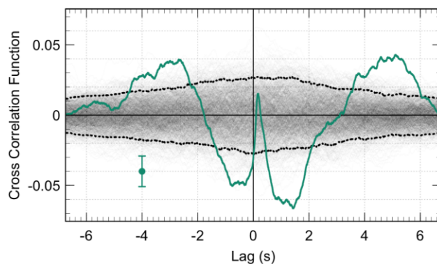
Figure A1. The g_s band versus X-ray CCF from epoch 4, averaged over 162 segments 10 s in size, is shown in green – similar to that seen in Fig. 3, but without binning. A representative error bar is plotted. The faded grey area is 1000 overlapping simulated correlation functions, and the black dotted lines are the 5 percent and 95 percent intervals of all the simulations. The feature at -3 s, noted in Section 4.4, is above this significance line. The -1 -s feature in epoch 6 was similarly found to be significant.
