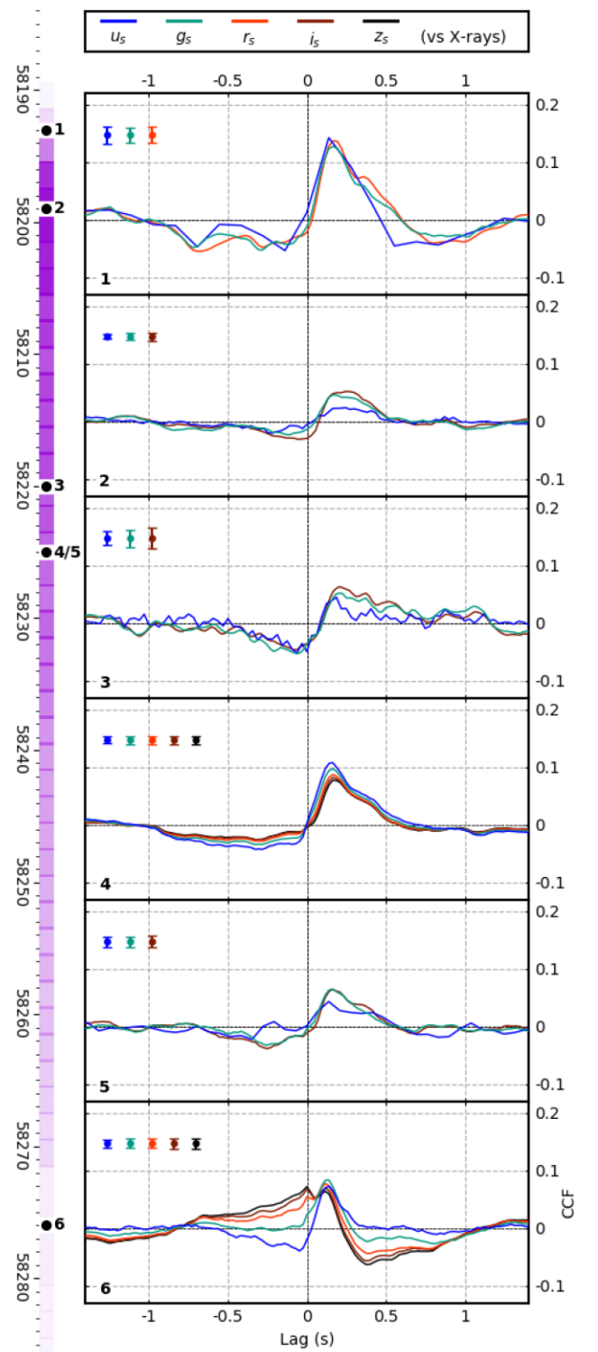
Figure 4. Same as in Fig. 3, but the CCFs are created from 2-s segments instead. This allows us to better compare the rapid variability and shows that the sub-second peak at positive lags is present in a similar place in every single band and epoch.
