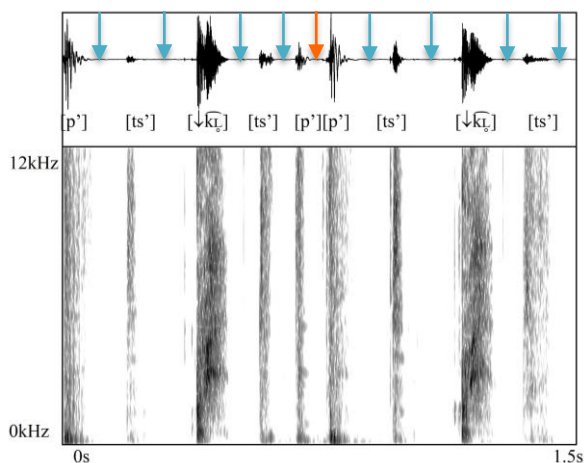
Figure 4: Waveform and spectrogram of the BP [p' ts' \downarrow k_l ts' p' p' ts' \downarrow k_l ts'] at 150 BPM.
