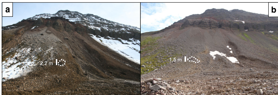
Fig. 8 Entrained talus deposits. a The erosional area as result of the entrainment of talus deposits by the initial mass (the picture was taken on 29th September 2012). b The same view of the erosional channel, partially re-filled by new talus material (the picture was taken in July 2015). Note the cone of debris as scale, resulting from the degradation of the ice-cemented block in panel a
