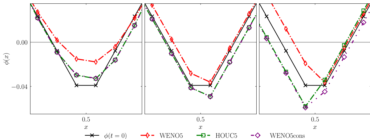
Figure 3: Numerical result of the advection 1D of the level set at a time t = 1.0 which corresponds to 200 advection step performed. Left: result without any reinitialization step. Middle: result when only one reinitialization procedure is applied at t = 1.0 . Right: result when the reinitialization procedure is applied every 10 advection steps.
