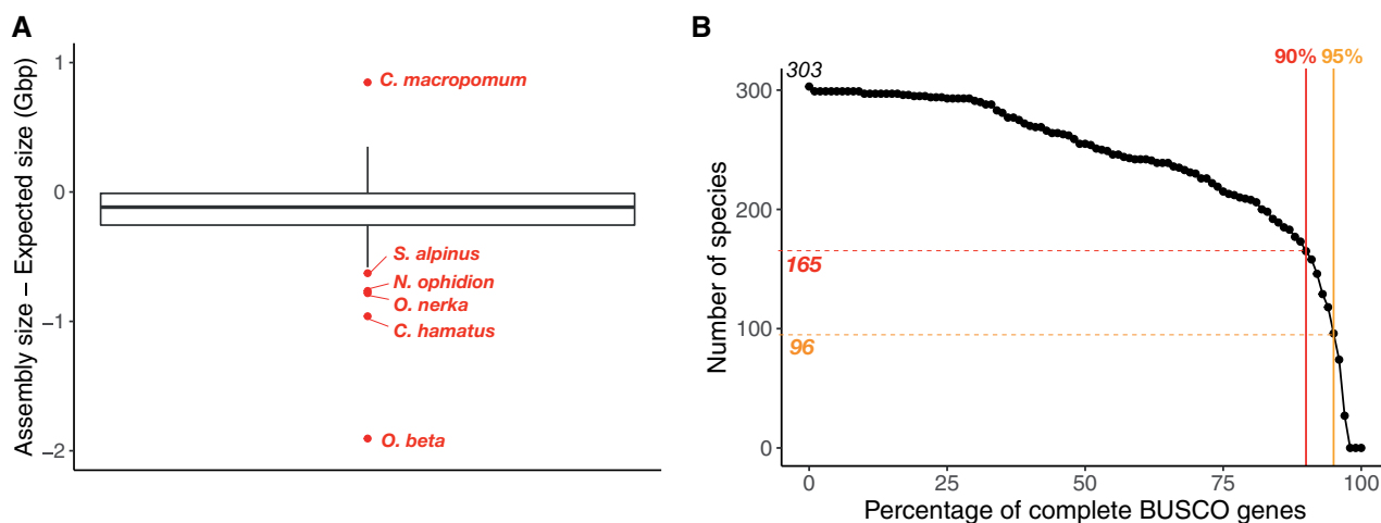
Fig. 1. Genome selection. (A) Congruence of genome assembly size and expected genome size based on haploid DNA content ( C\text{-value} \times 0.978 \times 10^9 ) for 309 actinopterygian fishes (307 teleosts and 2 nonteleosts); six incongruent estimates of genome size are shown in red and species names indicated (more details in supplementary fig. S3, Supplementary Material online ). (B) Number of genomes according to a completeness threshold (% of complete BUSCO genes). Out of 303 genomes with congruent estimates of genome size, 165 (163 teleosts and 2 nonteleosts) show a completeness > 90%, and 96 genomes (96 teleosts) a completeness > 95%.
