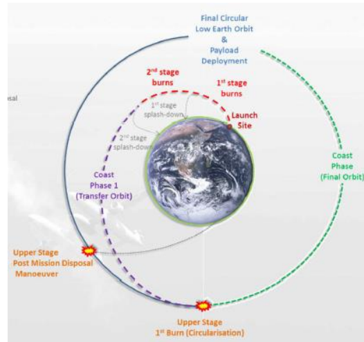
Fig. 14. Orbital module mission profile
