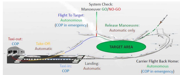
Fig. 7 ALTAIR CONOPS: COP (Carrier Operator) vs. Autonomous Operation
