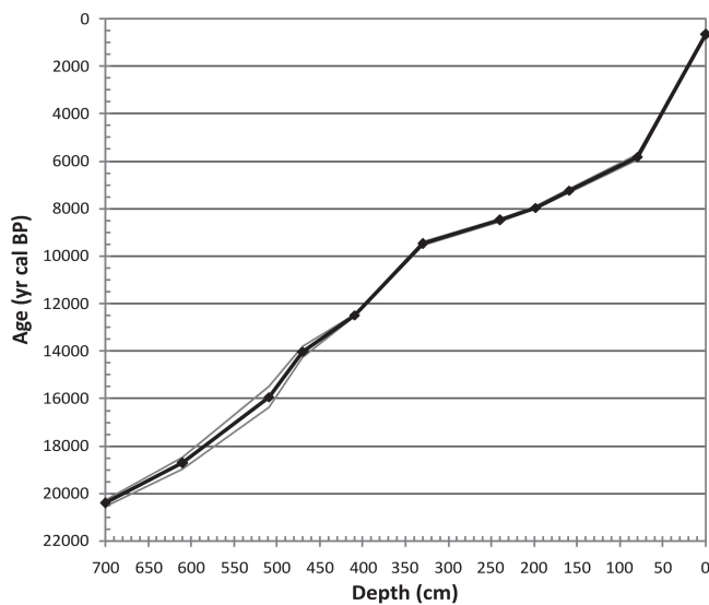
Fig. 2. Age-depth model for core MD04-2797CQ.
