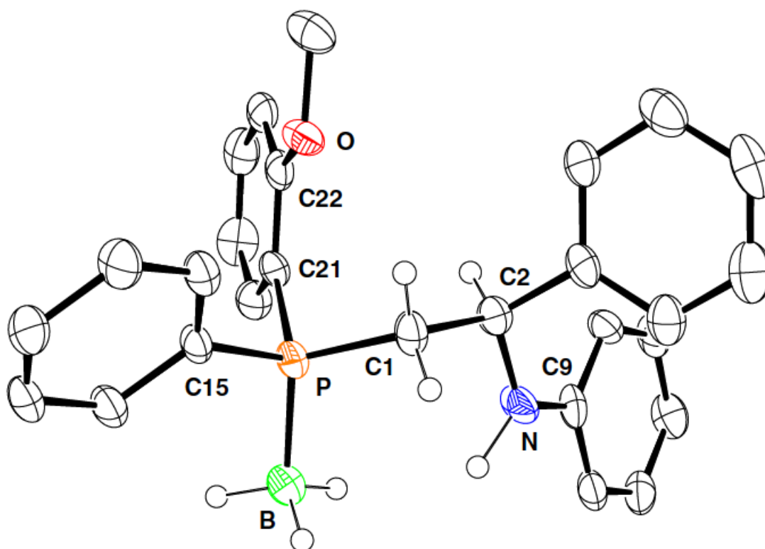
Figure 1. Crystal structure of the \beta -aminophosphine borane 6a . Selected bond lengths ( \text{\AA} ), angles ( ^\circ ), and dihedral angles ( ^\circ ): P–B 1.893(5), P–C(1) 1.822(4), C(1)–C(2) 1.542(5), C(2)–N 1.432(5), C(9)–N 1.398(5), C(15)–P–C(1) 104.7(2), C(15)–P–C(21) 108.6(2), C(15)–P–B 110.3(2), B–P–C(1) 113.1(2), C(1)–C(2)–N 110.0(3), C(1)–C(2)–C(3), C(2)–N–C(9) 122.9(3); B–P–C(21)–
