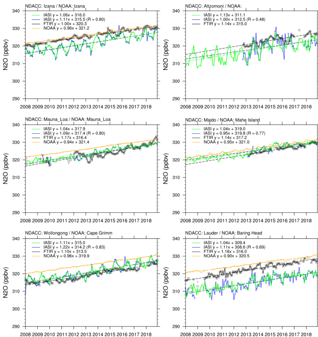
Figure 8. Same as Figure 7 at 6 NDACC stations for tropical and SH latitudes (Izana, Altzomoni, Mauna Loa, Maito, Wollongong, Lauder).
